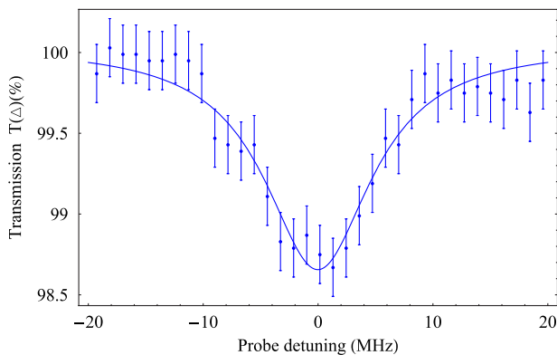
FIG. 2 (color online). Normalized power of a probe field transmitted through a single trapped Barium ion as a function of probe beam detuning. The transmission spectrum is fitted by a Lorentzian profile with a width of 11 MHz. The peak probe beam extinction is 1.35%. The error bars are derived from the rms value of the intensity fluctuations of the probe beam.
