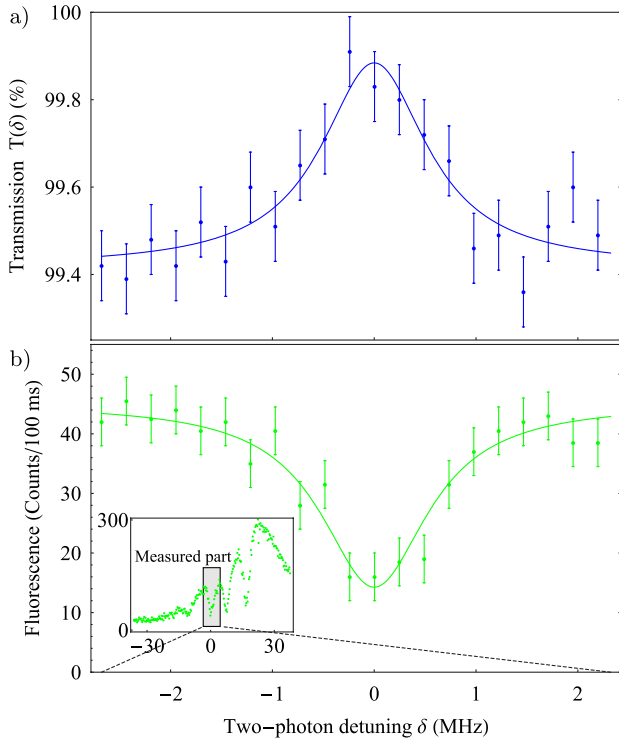
FIG. 3 (color online). Electromagnetically induced transparency and fluorescence spectra. (a) Normalized transmitted power of a probe field scattered by a single ion as a function of two-photon detuning (Here the control laser frequency is scanned). (b) Dark resonance in the fluorescence spectrum measured in the forward and backward directions. The inset shows a typical fluorescence spectrum with all four dark resonances. The EIT experiment was performed on the shaded part of the spectrum, with the levels as indicated Fig. 1(c).
