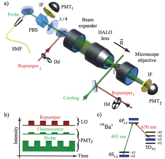
FIG. 1 (color online). (a) Schematic of the experimental setup. PBS: polarizing beam splitter, \lambda/4 : quarter-wave plate, IF: interference filter to select the green fluorescence, IM: intensity modulation, PMT: photomultiplier, and SMF: single-mode fiber. The ion is cooled by the cooling beam, while the repumper no. 1 recycles population from the D state manifold to the S_{1/2} to P_{1/2} transition. The probe beam is spatially adjusted to match part of the atomic dipole emission profile and is detected on the photomultiplier PMT 2 . In the EIT experiment, the probe field itself serves as a cooling beam and a copropagating repumper no. 2 is used instead. (b) Modulated detection scheme, see text for details. (c) A weak magnetic field \vec{B} lifts the energetic degeneracy of the Zeeman substates and creates an eight-level system. The levels marked as bold lines were employed in the EIT experiment.
