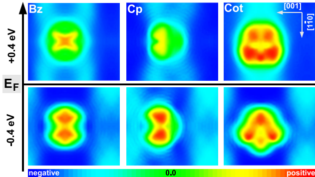
FIG. 2 (color online). The spin polarization at 2.5 Å above the Bz, Cp and Cot molecules adsorbed on the 2ML Fe/W(110) ( 15.85 \text{ \AA} \times 13.45 \text{ \AA} ) surface plotted for occupied ( [-0.4, 0.0] eV) and unoccupied ( [0.0, +0.4] eV) energy intervals around the Fermi level. All the organic molecules show a high, locally varying spin polarization ranging from attenuation to inversion with respect to the ferromagnetic Fe film. As compared to Bz, the strongly interacting Cp molecule shows an amplification of the inversion of the spin polarization below Fermi level, while the Cot molecule shows a strong amplification of the inversion of the spin polarization for both occupied and unoccupied states around the Fermi level due to a higher number of p_z interacting electrons.
