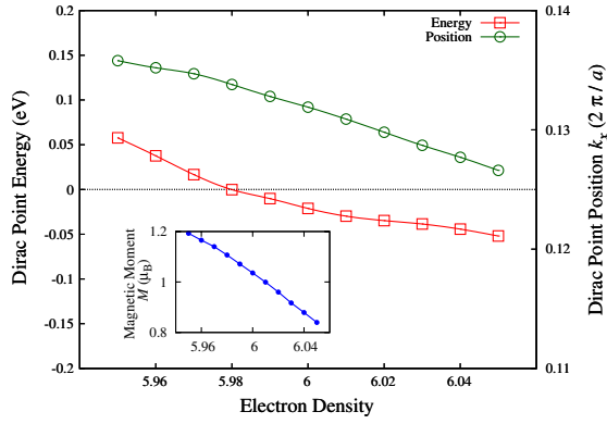
FIG. 4 (color online). The electron density dependence of the Dirac point and the Dirac point position in the Brillouin zone denoted by (k_x, 0) . The inset shows the electron density dependence of the magnetic moment.
