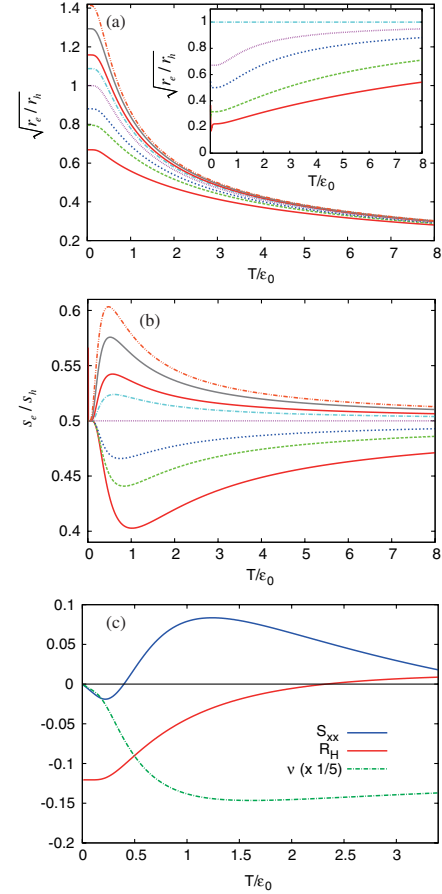
FIG. 3 (color online). The temperature dependence of the ratios \sqrt{r_e/r_h} (a) and s_e/s_h (b) for different values of the density ratio n_r . ( n_r = 1.0, 0.70, 0.45, 0.35, 0.25, 0.15, 0.10, 0.05 from top to bottom.) The inset in (a) shows the temperature dependence of \sqrt{r_e/r_h} for conventional energy dispersions. ( n_r = 1.0, 0.45, 0.25, 0.10, 0.05 from top to bottom.) (c) The temperature dependence of the Hall coefficient, the Seebeck coefficient, and the Nernst coefficient, which are normalized by (2\pi a^2/|e|) \times (\hbar v/\varepsilon_0 a)^2 , k_B/|e| , and [k_B a^2/(2\pi\hbar)](\hbar v/\varepsilon_0 a)(v\tau_D/a) , respectively, with k_B the Boltzmann constant.
