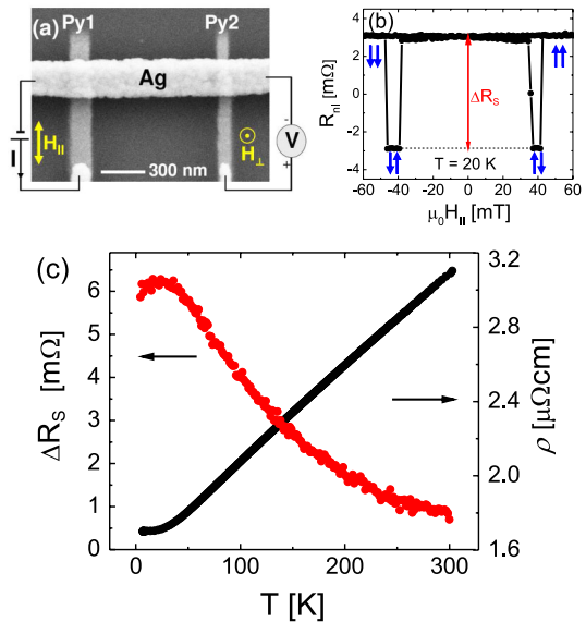
FIG. 1 (color online). (a) An SEM image of a Py/Ag LSV device adapted to show the nonlocal measurement configuration. Also shown are the directions of H_{||} and H_{\perp} applied in NLSV and Hanle effect measurements, respectively. (b) R_{nl} vs H_{||} at 20 K. Corresponding M orientations of the Py electrodes are shown as blue (dark gray) arrows, while the total \Delta R_s signal is highlighted in red (medium gray). (c) T dependencies of \Delta R_s and \rho .
