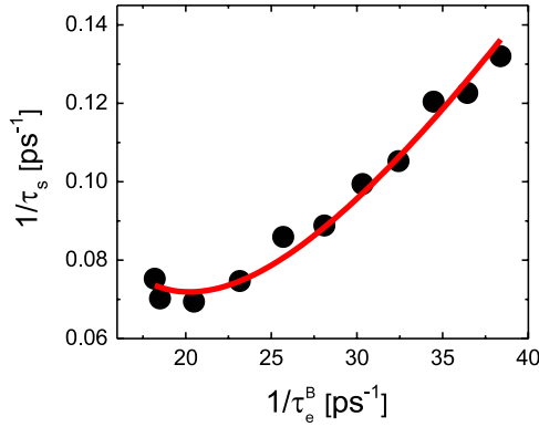
FIG. 4 (color online). Dependence of spin relaxation rate in the Ag wire on the bulk momentum relaxation rate (black circles). The fit to the data according to Eq. (7) is shown as a red line.
