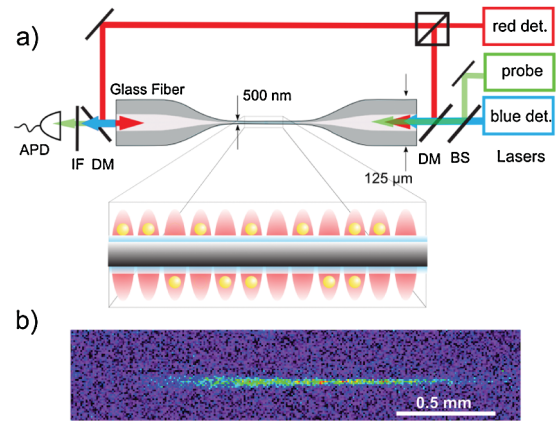
FIG. 2 (color). (a) Experimental setup of the fiber-based atom trap. The blue-detuned running wave in combination with the red-detuned standing wave creates the trapping potential. A resonant laser is used for probing the atoms via the evanescent field. (b) Fluorescence image of the trapped atomic ensemble.
