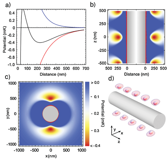
FIG. 1 (color). (a) (black line) Potential as a function of distance from the surface of a 500-nm diameter nanofiber for a ground state cesium atom induced by a two-color evanescent field plus the van der Waals potential. The red and blue lines show the individual light induced potentials for a red- and blue-detuned field at 1064 and 780 nm, respectively. We assumed a power of P_{\text{red}} = 2 \times 2.2 mW (standing wave) and P_{\text{blue}} = 25 mW and orthogonal linear polarization of the red and blue fields. (b) Contour plots of the same potential as in (a). The red-detuned standing wave ensures axial confinement. (c) Azimuthal plot of the same potential as in (a) and (b). The planes of the plots in (a)–(c) are chosen to include the trapping minima. (d) Contour plot of the resulting array of trapping sites on both sides of the fiber showing equipotential surfaces 40 and 125 \mu\text{K} above the trapping minimum.
