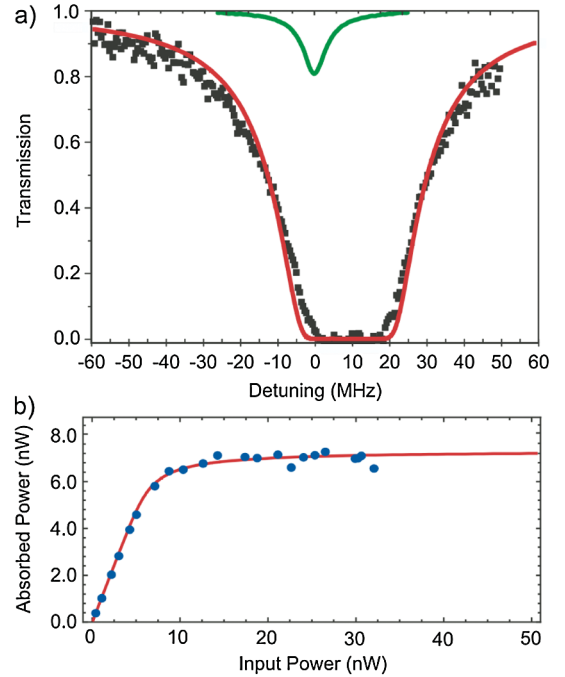
FIG. 3 (color). (a) Transmission spectrum of the probe beam through the nanofiber after loading the trap (black squares). For reference, the spectrum of the MOT cloud (green line) is plotted. The red line is a theoretical fit, see text. (b) Saturation measurement (blue circles) yielding the number of trapped atoms. The red line is a theoretical fit, see text.
