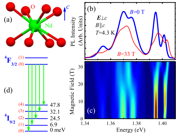
FIG. 1 (color online). (a) Local square antiprismatic environment of the \text{Nd}^{3+} centers. (b) PL spectra at 4.3 K. (c) Magnetic field dependence of the PL at 4.3 K for \vec{B} \parallel c . Gray scale (color) denotes intensity: dark (blue) is low; bright (red) is high. (d) Energy level diagram of the ^4F_{3/2} \rightarrow ^4I_{9/2} emission, with crystal field splitting extracted from the peak positions in (b).
