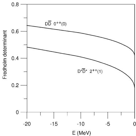
FIG. 2. Fredholm determinant of the most attractive J^{PC}(I) channels for the D\bar{D} and D^*\bar{D}^* systems.
