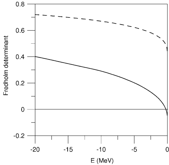
FIG. 1. Fredholm determinant for the J^{PC}(I) = 1^{++}(0) D\bar{D}^* system. Solid (dashed) line: results with (without) coupling to the J/\Psi\omega channel.
