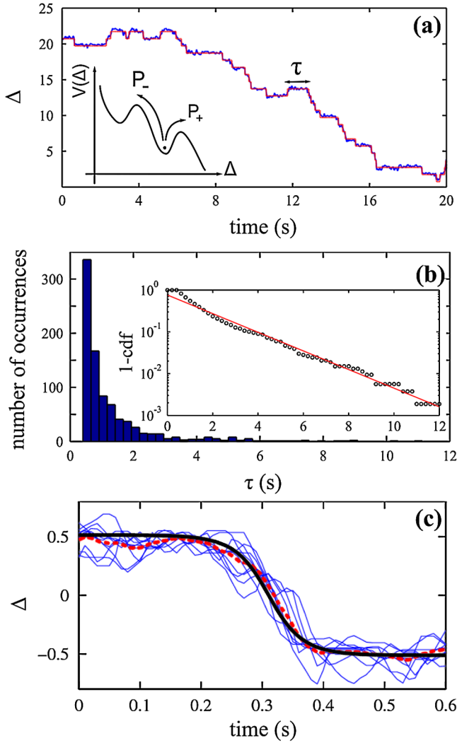
FIG. 3 (color online). Dynamics and statistics of phase slips. (a) Long time series of \Delta(t) illustrating forward and backward slips. Inset: sketch of the tilted washboard potential used in the model. (b) Probability distribution of synchronization times and its cumulative distribution function (cdf) showing approximate exponential decay. (c) \Delta(t) for 10 slips events, the average slip (dashed line) and the integrated trajectory from the deterministic part of the model (solid line) for \delta\nu/\bar{\nu} = 0.004 , \bar{\nu} = 47 Hz, and \epsilon/\bar{\nu} = 0.015 ; \tau_{\text{slip}} \sim 0.22 s.
