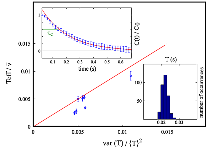
FIG. 4 (color online). Comparison of single flagellum noise levels before (y axis) and after (x axis) partial deflagellation. In the latter case, the noise can be extracted from the distribution of beating periods (lower inset), and compared to the value estimated from the autocorrelation of the coupled dynamics (upper inset). Only experiments in which the isolated flagellum had a long period of uniform behavior are shown (7 out of 14).
