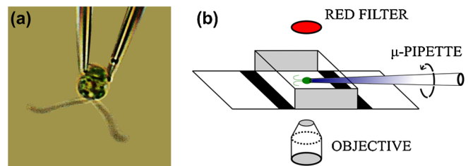
FIG. 1 (color online). Experimental system. (a) A single cell of Chlamydomonas reinhardtii held on a micropipette. (b) Schematic of apparatus for visualization and micromanipulation of cells.
