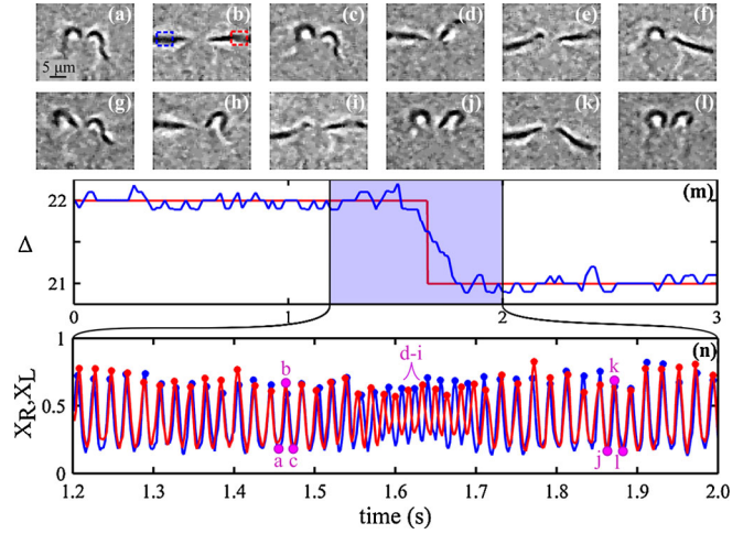
FIG. 2 (color online). A phase slip in the beating of C. reinhardtii flagella. (a)–(l) Individual image-processed movie frames at times indicated in panel n . (m) Phase difference \Delta(t) between flagella as a function of time. (n) Extracted signals from the interrogation areas [seen in (b)] near each of the two flagella.
