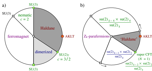
FIG. 1 (color online). Phase diagrams of the “biquadratic” spin-1 chain for (a) \text{SU}(2) and (b) \text{su}(2)_k with k \geq 5 . Projections onto the triplet ( j = 1 ) and quintuplet ( j = 2 ) states are parametrized by an angle \theta as J_1 = -\sin(\theta) and J_2 = \cos(\theta) .
