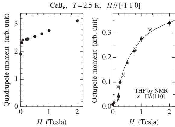
FIG. 4. Magnetic-field dependences of the AFQ and AFO moments deduced from the symmetric E1 and asymmetric E2 intensities in Fig. 2. The solid line is a guide for the eye. The crosses represent the THF as deduced from NMR.
