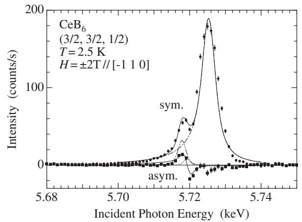
FIG. 3. X-ray energy dependence of the symmetric and asymmetric components deduced from the data for \pm 2 T. The solid lines are the fits to the data with Lorentzian components. The single-dotted, double-dotted, and dotted lines represent the 1st, 2nd, and 3rd term in Eq. (4), respectively.
