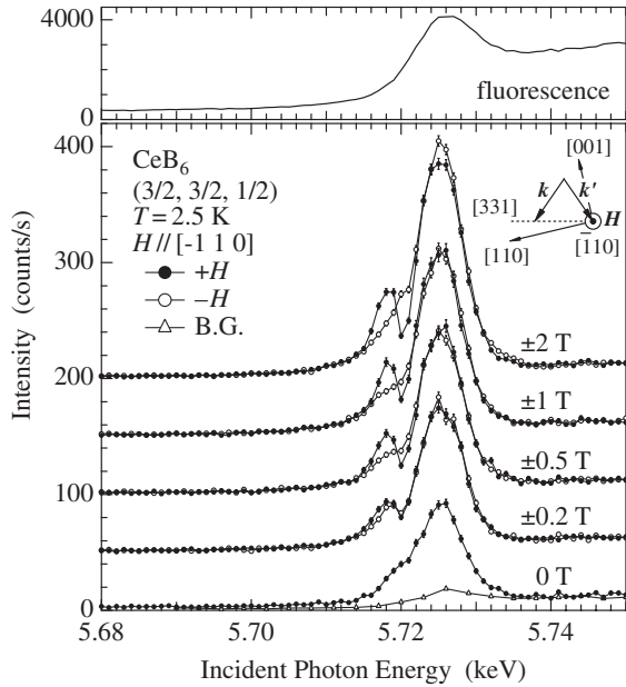
FIG. 1. Top: Fluorescence spectrum of CeB 6 . Bottom: X-ray energy spectra of the (\frac{3}{2}, \frac{3}{2}, \frac{1}{2}) superlattice reflection in magnetic fields with reversed directions. The triangle shows the background due to the fluorescence.
