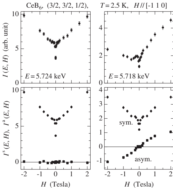
FIG. 2. Top: Magnetic-field dependence of the integrated intensity of the (\frac{3}{2}, \frac{3}{2}, \frac{1}{2}) resonant Bragg diffraction measured at E = 5.724 (left) and 5.718 keV (right), corresponding to the E1 and E2 processes, respectively. Bottom: Symmetric (circles) and asymmetric (squares) components of the intensity for the respective processes.
