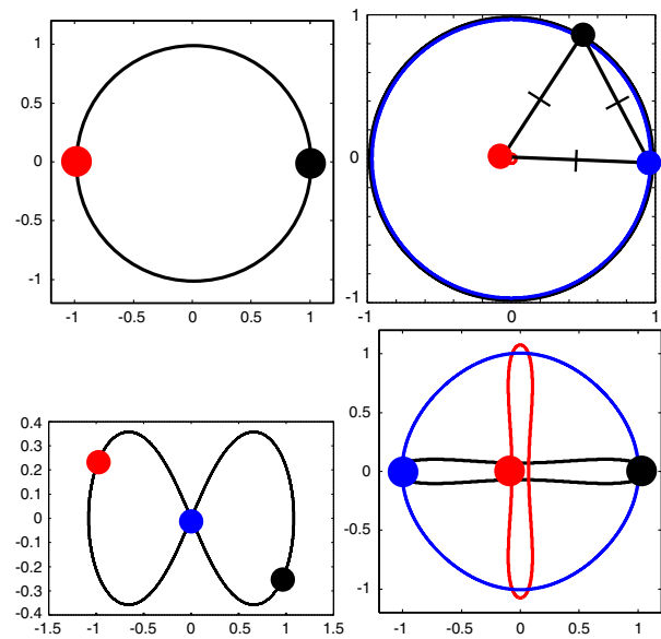
FIG. 1 (color online). Orbital shapes. (a) Top left: circular orbit for two-body system as a reference. (b) Top right: triangle solution by Lagrange. (c) Bottom right: crisscross orbit by Henon. (d) Bottom left: figure eight trajectory by Moore.
