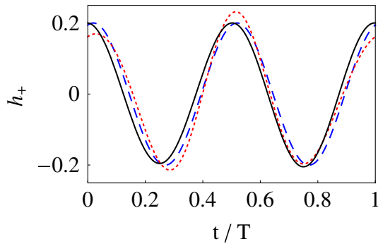
FIG. 4 (color online). Gravitational wave forms in arbitrary units for a binary (solid black curve) with m_1:m_2 = 2:3 and a Lagrange solution (dotted red curve) with m_1:m_2:m_3 = 1:2:3 , where both the quadrupole and octupole parts are included. As a reference, we give the quadrupolar wave forms from the same sources (dashed blue curve). We assume a = 100m_{\text{tot}} in order to exaggerate a correction by the octupole (nearly 10% expected in this figure). One can see that the dashed blue curve will overlap with the solid black one after they are shifted by choosing the initial phase. This coincidence is because the octupolar waves for the binary case are proportional to the mass difference [38] and thus relatively small in this figure.
