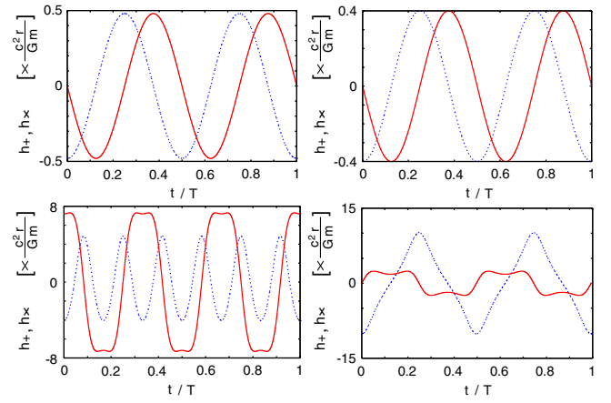
FIG. 2 (color online). Gravitational wave forms in arbitrary units ( T = orbital period). Dotted blue and solid red curves denote + and \times modes, respectively. (a) Top left: Gravitational wave forms by binary system with a mass ratio of 2:3 in circular motion. (b) Top right: Lagrange's triangle solution for a mass ratio of 1:2:3. (c) Bottom right: Henon's crisscross. (d) Bottom left: Moore's figure eight. Crisscross and figure eight have larger curvatures in the orbital shapes than Keplerian and Lagrangian orbits, which lead to larger acceleration of the particles and thus relatively stronger radiation.
