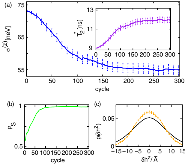
FIG. 2 (color online). (a) Averaged Overhauser field fluctuations \sigma^{(z)} and electron spin decoherence T_2^* = \hbar/\sigma^{(z)} (upper inset) as a function of the number of performed cycles. (b) Singlet return probability P_S as a function of the number of performed cycles. Error bars are smaller than line thickness. (c) Initial (black) and final (orange) averaged probability distribution of the nuclear spin eigenstates of \delta h^2 . Repeated cycles narrow the distribution, showing a reduction of \sigma^{(z)} .
