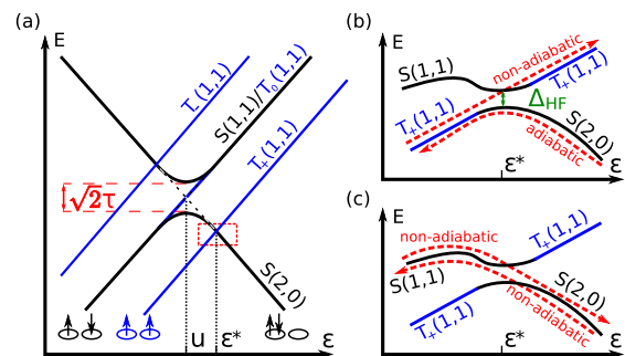
FIG. 1 (color online). (a) Energy diagram for the relevant states of the double quantum dot as a function of the bias \epsilon . (b) The hyperfine interaction allows for flip-flop processes that open a gap \Delta_{HF} at the S - T_+ crossing. Driving the system slowly from S(2,0) can result either in an adiabatic (b) or a nonadiabatic (c) transition. Driving the system back very fast results in a non-adiabatic passage to two distinguishable charge states.
