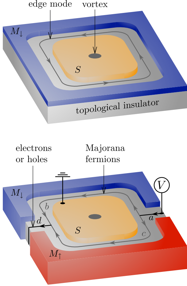
FIG. 1 (color online). Three-dimensional topological insulator in proximity to ferromagnets with opposite polarization ( M_{\uparrow} and M_{\downarrow} ) and to a superconductor ( S ). The top panel shows a single chiral Majorana mode along the edge between superconductor and ferromagnet. This mode is charge neutral, so it cannot be detected electrically. The Mach-Zehnder interferometer in the bottom panel converts a charged current along the domain wall into a neutral current along the superconductor (and vice versa). This allows for electrical detection of the parity of the number of enclosed vortices, as explained in the text.
