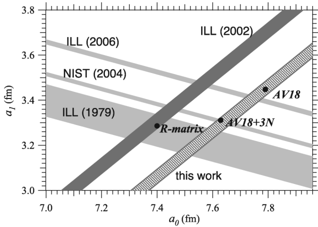
FIG. 4. Summary of the triplet and singlet n - ^3\text{He} free neutron scattering lengths (real parts). The three coherent (unpolarized) measurements labeled ILL (1979) [26], NIST (2004) [11], and ILL (2006) [12] used neutron interferometry. The incoherent (polarized) measurement ILL (2002) [13] used pseudomagnetic spin rotation. The three theoretical points shown are from Ref. [24].
