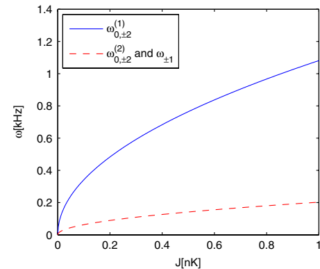
FIG. 3 (color online). The frequencies of pseudo Goldstone modes as a function of coupling parameter J in the case of cyclic phase. The dependence on J is similar to the case in antiferromagnetic phase. However, there are two degenerate modes \omega_{0, \pm 2}^{(2)} and \omega_{\pm 1} in this case, which are originated from the two degenerate Bogoliubov modes in the uncoupled system.
