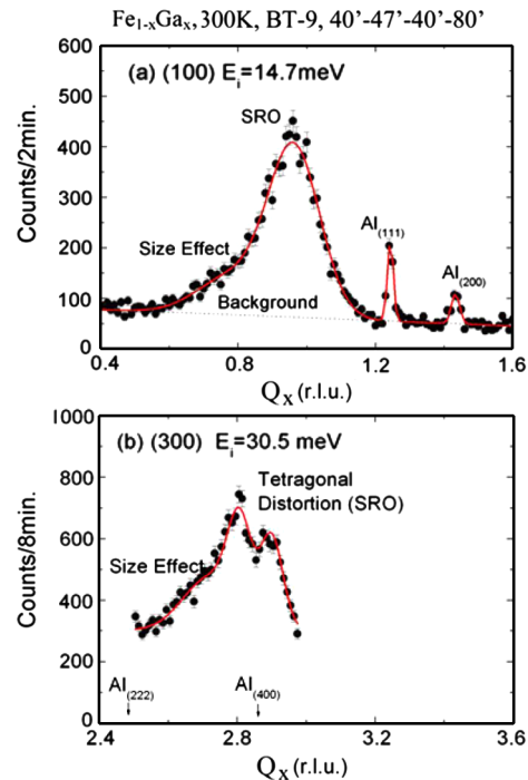
FIG. 3 (color online). Diffuse scattering profiles for furnace-cooled \text{Fe}_{0.81}\text{Ga}_{0.19} at 300 K measured on BT9 near (a) (100) and (b) (300). The black dotted line in (a) represents the background. The solid lines through the data points in (a) and (b) represent fits using multi-Gaussian functions. The sharp peaks near q = 1.2 and 1.45 in (a) are the (111) and (200) reflections from the Al wire used to mount the sample: The positions of the Al (222) and (400) reflections are indicated in the (300) profile in (b).
