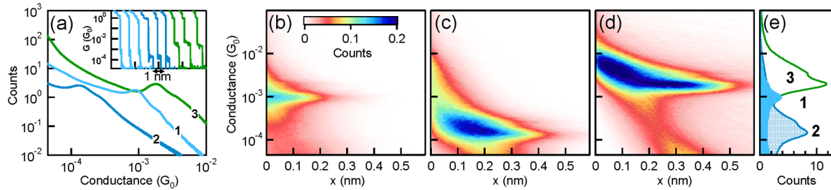
FIG. 1 (color online). (a) Normalized linear conductance histograms of 1,4-butanediamine (1, bin size 10^{-5}G_0 ), 1,6-hexanediamine (2, bin size 10^{-6}G_0 ), and 1,4-bis(dimethylphosphino)butane (3, bin size 10^{-5}G_0 ). Inset: Sample conductance traces (offset horizontally for clarity) that show a molecular step for each molecule. (b)–(d) Normalized 2D histograms for molecules 1, 2, and 3, respectively (100 bin/decade against 0.007 nm/bin). (e) Normalized log-bin conductance histograms for 1, 2, and 3.
