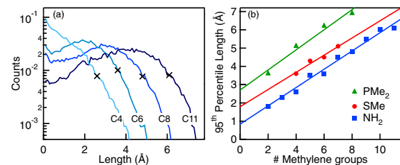
FIG. 2 (color online). (a) Conductance step length distribution for diamino alkanes with 4, 6, 8, and 11 \text{CH}_2 groups in the chain. Crosses indicate the 95th percentile for each distribution. (b) Conductance step length (95th percentile) as a function of the number of \text{CH}_2 groups for alkanes with the three links studied.
