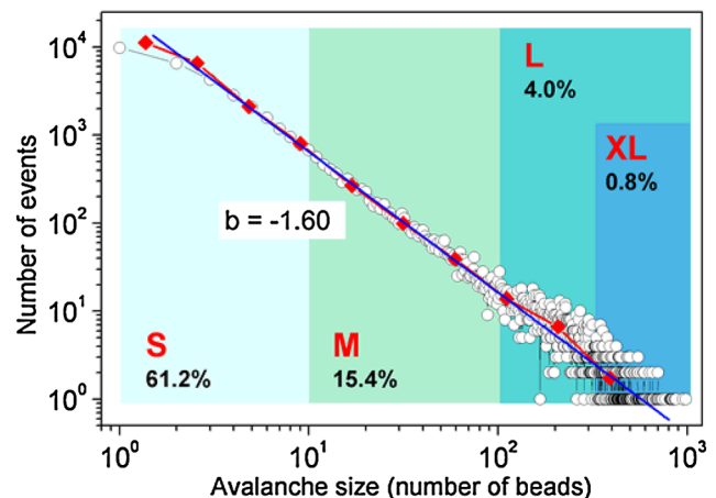
FIG. 1 (color online). Distribution of avalanche size (open circles). These points have been averaged with a logarithmic binning (diamonds). Avalanches are classified as small (S), medium (M), large (L), and very large (XL) considering logarithmic bins. The percentage of every type of avalanche related to the total number of dropping events is also displayed.
