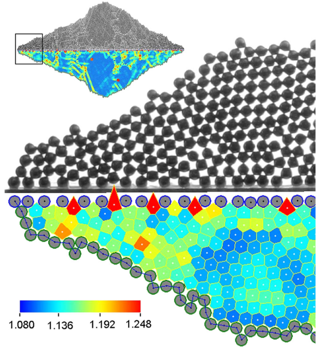
FIG. 3 (color online). Internal structure of a pile. Close-up of a portion of the pile with a reflection (below) in the space of the shape factor \zeta . After finding the center of the beads and making a voronoi triangulation for the internal ones (i.e., excluding those in the base and those joined with a line at the pile’s surface) we define \zeta = C^2/4\pi S , where C is the perimeter and S the area of each voronoi cell. The shape factor \zeta is a measure of the local disorder in the pile [for example for a regular hexagon \zeta = 1.103 (highest order in the pile) and for a square \zeta = 1.273 ]. Inset: The whole pile, where a rectangle indicates the close-up area. Notice the small values of \zeta at the center of the pile, indicating hexagonal packing which results from the “thermal” effect of beads being added from above.
