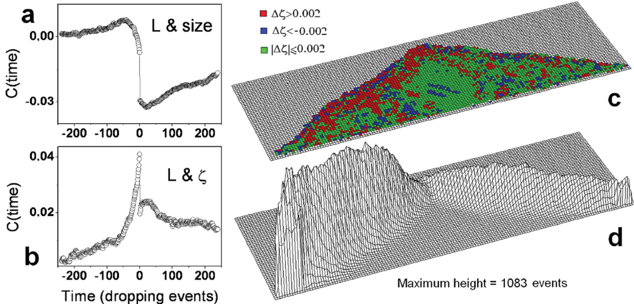
FIG. 4 (color). Correlation between avalanches and internal structure. (a) Temporal correlation between the large avalanches and the size of the system. (b) Temporal correlation between the large avalanches and the average shape factor \zeta . (c) Difference between the local averages of the \zeta values at one step before a large avalanche and at 50 steps before a large avalanche. Red indicates that the disorder increases, blue an increase in the order, and green displays no variations in \zeta . A cursory inspection shows that the red color predominates over the blue. The cumulative number of sites involved in large avalanches is displayed at (d). The match between the red color in (c), and the landscape in (d), corroborates that on average, the pile suffers an increment of the disorder before a large avalanche takes place.
