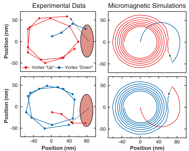
FIG. 2 (color). The left-hand panels show separate plots of the trajectories of both the up and down vortex, as visible in the frames of Fig. 1(c). The hatched area replaces the vortex position at the assumed switching time, where it could not be accurately tracked. In comparison, the right-hand panels show the corresponding micromagnetic simulation using parameters derived from the observed sample, under identical excitation, with an arrow connecting the positions of the vortex before and after switching.
