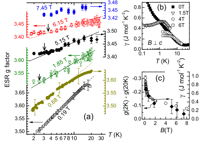
FIG. 2 (color online). (a) g(T) dependence for B \perp c at \nu = 9, 34, 93, 249, 297, and 360 GHz (from bottom to top), which correspond to resonance fields as indicated. Arrows indicate a crossover from a -\ln T to g = \text{const} behavior. (b) T dependence of the Sommerfeld coefficient \gamma at different magnetic fields (Ref. [5]). (c) Field dependence of low temperature \gamma (Ref. [5]) and g shift between 20 K and 2 K.
