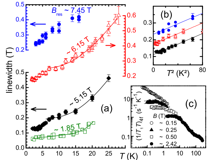
FIG. 3 (color online). (a) T dependence of the linewidth \Delta B for B \perp c at \nu = 93 (squares), 249 (diamonds), 297 (triangles), and 360 GHz (circles). Solid lines are fits (see the text). (b) Corresponding low- T data in the representation \Delta B vs T^2 . Solid lines are fits to the T^2 dependence. (c) T dependence of ^{29}\text{Si} relaxation rate 1/(T_1 T) from Ref. [3].
