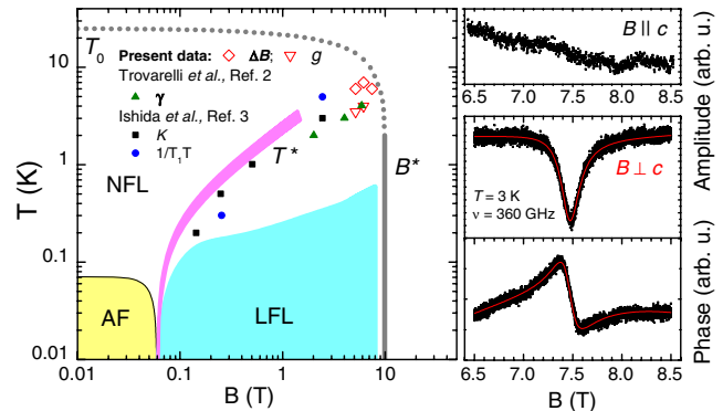
FIG. 1 (color online). Left: Schematic phase diagram of \text{YbRh}_2\text{Si}_2 for B \perp c from Ref. [1]. Dashed and solid gray lines delineate the region of heavy QP behavior confined to the region T < T_0 and B < B^* [2,4,5]. The LFL region denotes the T - B domain where the resistivity follows LFL behavior \rho \propto T^2 . The broad (pink online) line T^* depicts the position of crossover in the isothermal Hall resistance, magnetostriction, magnetization, and longitudinal resistivity. Closed symbols depict T(B) -crossover temperatures below which specific heat ( \gamma ) [2] and ^{29}\text{Si} -NMR quantities [ K and 1/(T_1T) ] [3] become T independent. Open symbols display crossover temperatures from HF ESR g(T, B) and \Delta B(T, B) dependences (see text). Right: A representative HF ESR signal for the B \perp c axis. Absorptive (amplitude) and dispersive (phase shift) parts of the ESR signal (noisy curves) are simultaneously fitted to a Lorentzian function (solid lines). No signal can be observed for the B \parallel c axis, suggesting a strong g factor anisotropy.
