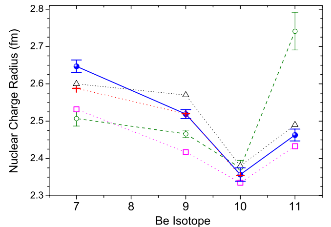
FIG. 3 (color online). Experimental charge radii of beryllium isotopes from isotope-shift measurements ( \bullet ) compared with values from interaction-shift cross-section measurements ( \circ ) and theoretical predictions: Greens-function Monte Carlo calculations ( \+ ) [2,24], fermionic molecular dynamics ( \Delta ) [25], ab initio no-core shell model ( \square ) [13,26,27].
