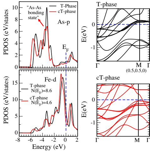
FIG. 2 (color online). The projected electronic density of states (PDOS) for As p -orbital (top-left) and Fe-d orbital (bottom left) for T - and cT -phases. The right two panels show the band structure along \Gamma - M - \Gamma . The As-As p_z -bonding orbital is indicated by the arrow on the top left panel, and it is shown in Fig. 3.
