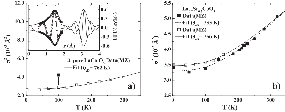
FIG. 2. (a) \sigma^2(T) for \text{LaCoO}_3 and the correlated Debye fit. The inset is an example of 4 K r -space data (solid line) and a fit to Co-O first peak (open circle); the Fourier transform (FT) range is 3.3\text{--}12.0 \text{ \AA}^{-1} with a Gaussian broadening of 0.3 \text{ \AA}^{-1} , and the r -space fit range is 1.1 to 1.7 \text{ \AA} . Note that we are fitting to the fast oscillating real and imaginary (not shown) parts of the FT. A good fit is obtained from 0.7\text{--}1.8 \text{ \AA} . (b) \sigma^2(T) for the \text{La}_{0.7}\text{Sr}_{0.3}\text{CoO}_3 JM samples. The solid squares represent the data from the first measurement, and open squares represent the data from the second measurement showing consistency between measurements taken a year apart; the dashed line is the correlated Debye fit for the first experiment data, while the solid line is the fit for the second experiment data. The solid symbol in (a) shows the increase in \sigma^2 if a 3-peak splitting occurs near 100 \text{ K} .
