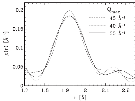
FIG. 4. \rho(r) obtained from the scattering data on LCO using different Q_{\max} at T = 200 K. Although a small peak can be seen between 2.1 and 2.2 Å, its position changes with Q_{\max} and does not indicate a real bond length in this r range.
