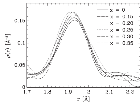
FIG. 3. \rho(r) for all the samples at T = 300 \text{ K} with Q_{\text{max}} = 35 \text{ \AA}^{-1} . The large peak represents a Co-O bond length of 1.92 \text{ \AA} . There is little evidence for the peak previously reported [11] at 2.15 \text{ \AA} .
