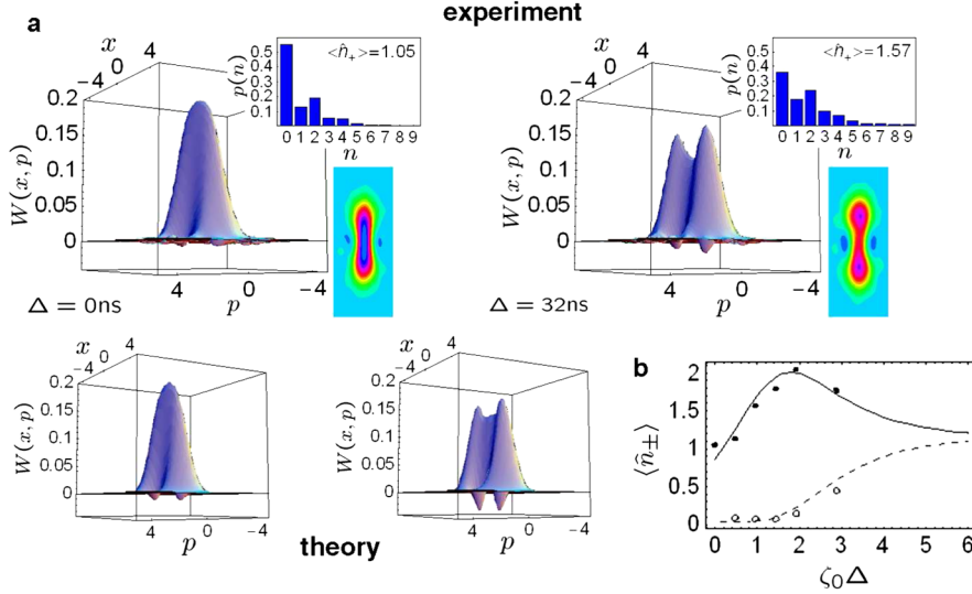
FIG. 4 (color online). (a) Wigner functions of the state \hat{\rho}_+ in mode \Psi_+ for \Delta = 0 ns ( \zeta_0 \Delta = 0 , left) and \Delta = 32 ns ( \zeta_0 \Delta = 0.90 , right). Upper row: experimental Wigner functions ( W(x, p) ), their contours, and photon-number distributions ( p(n) ). Lower row: model calculation of the Wigner functions. (b) Average photon numbers in modes \Psi_\pm . Upper (filled) plots: experimental \langle \hat{n}_+ \rangle with \Delta = 0, 32, 48, 64, 96 ns, from left to right. Lower (unfilled) plots: experimental \langle \hat{n}_- \rangle with \Delta = 32, 48, 64, 96 ns, from left to right. Solid ( \langle \hat{n}_+ \rangle ) and dashed ( \langle \hat{n}_- \rangle ) lines are the theoretical predictions including 15% optical loss.
