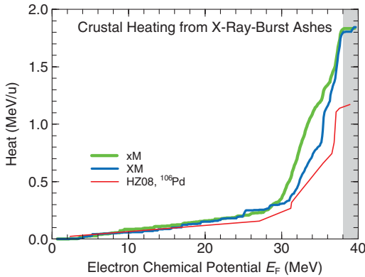
FIG. 2 (color). Crustal heating in our MCP model for ICC (XRB ashes from [3]) from NS accreting 5% solar ( x ) and solar metallicities ( X ) at the accretion rate M = 0.1\dot{m}_{\text{Edd}} characteristic of Superburst progenitors (accretion at the Eddington limit is \dot{m}_{\text{Edd}} \approx 8.85 \times 10^4 \text{ g cm}^{-2} \text{ s}^{-1} ). Also plotted are OCP heating from [14] for the ICC comprised of ^{106}\text{Pd} . ICC from multizone XRB model xM : Peak A \sim 100 – 110 (very similar to the 1-zone rp process products of [4] and also to an ICC of pure ^{106}\text{Pd} in the OCP model of [14]). ICC from model XM : A bimodal abundance distribution with significant pre-Fe-peak abundance, and also in A \sim 60 – 80 .
