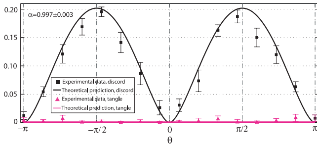
FIG. 4 (color online). Nonclassical correlations generated by our DQC1 algorithm. Discord and tangle are derived from the reconstructed density matrices measured at the algorithm output for \alpha = 0.997 \pm 0.003 [Fig. 3(a)]. Discord is calculated by optimizing over all 1-qubit projective measurements on qubit c , Fig. 1 [26]. Theoretical predictions are calculated using measured input states and assuming perfect circuit operation.
