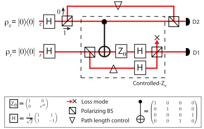
FIG. 2 (color online). Experimental schematic. Qubits at the input and output are encoded in the polarization of single photons ( |0\rangle = |H\rangle , |1\rangle = |V\rangle , horizontal and vertical). Coincident measurement of single photons at fiber-coupled counting modules (D1, D2) signals a successful run of the algorithm. Photons are generated via spontaneous parametric down conversion of a frequency-doubled mode-locked Ti:sapphire laser (820 nm \rightarrow 410 nm, \Delta\tau = 80 fs at 82 MHz) pumping a type-I 2 mm \text{BiB}_3\text{O}_6 crystal; filtered to 820 \pm 1.5 nm; collected into two single-mode optical fibers; then injected into free-space modes c and r . With 100 mW at 410 nm, we measure a twofold coincidence rate at the output of the optical circuit of \approx 100 \text{ s}^{-1} . Interferometers are realized using calcite beam displacer pairs, rotating one displacer of a pair about an axis perpendicular to the plane defined by the two paths enables relative path length control. The two-qubit gate is realized nondeterministically as described in Ref. [29].
