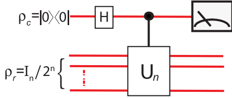
FIG. 1 (color online). Algorithm for estimating the normalized trace of the unitary operator U_n , using deterministic quantum computing with 1-qubit (DQC1). I_n is the n -qubit identity. Repeated running of the circuit and measurement of qubit c in the Pauli X ( Y ) basis yields an estimate of the corresponding expectation value, from which one can derive the real (imaginary) part of the normalized trace ( \text{Tr}[U_n]/2^n ).
