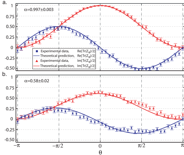
FIG. 3 (color online). Algorithm output. Real (blue or dark gray) and imaginary (red or gray) parts of the normalized-trace measured for two values of \alpha , over a range of \theta , Eq. (4). \alpha is the degree of purity of the control qubit as described in the text. \langle X \rangle is estimated by counting the number of coincident photon pairs ( N_{\pm} ) when projecting qubit c into the states |\pm\rangle = (|0\rangle \pm |1\rangle)/\sqrt{2} , over 10 sec. Then \langle X \rangle = (N_+ - N_-)/(N_+ + N_-) . The same technique is used to estimate \langle Y \rangle , but in this case we project into the states |\pm i\rangle = (|0\rangle \pm i|1\rangle)/\sqrt{2} . All error bars are calculated assuming Poissonian uncertainties in the counting statistics. We use the standard definition for a reduced- \chi^2 calculation [22], allowing for 3 degrees of freedom [the real and imaginary parts of the trace are simple trigonometric functions defined by an amplitude, frequency and phase, Eq. (3)]. Note that the goal of the algorithm is to return the normalized trace. The full trace is not required for the DQC1 applications mentioned in the introduction.
