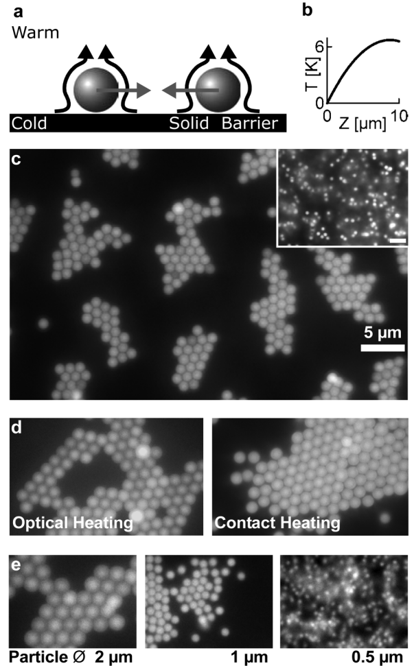
FIG. 2. Thermophoretic crystallization . (a) In a strong temperature gradient, particles move ballistically to the cold surface (side view). The persisting slip flow is deflected by the surface and leads to mutual hydrodynamic attraction. (b) Temperature profile. (c) Colloidal crystals of 1\ \mu\text{m} polystyrene particles on a cold surface for positive Soret coefficients (view from the top after 20 s of heating). Inset: Before temperature application. (d) Crystals form equally well for a contact heated chamber without laser irradiation ( 2\ \mu\text{m} particles). (e) At a fixed temperature gradient of 0.28\ \text{K}/\mu\text{m} , crystallization strongly depends on the Soret coefficient, following the threshold condition of Eq. (1). See supplemental material [34].
