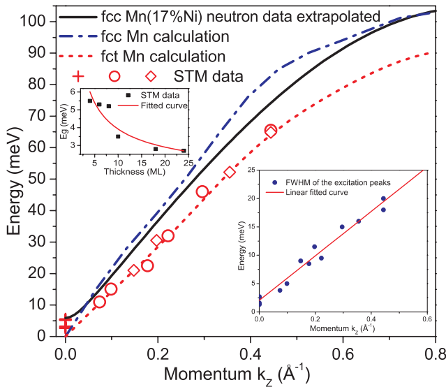
FIG. 3 (color online). Spin wave dispersion of \gamma -Mn. The notations (cross, circle, parallelogram) of STM data are the same as in Fig. 2. The extrapolated neutron scattering data is from [18]. The fcc and fct Mn dispersions were obtained by ab initio calculations. The upper inset gives the gap E_g as a function of film thickness (see text) and the lower, the FWHM as a function of k .
