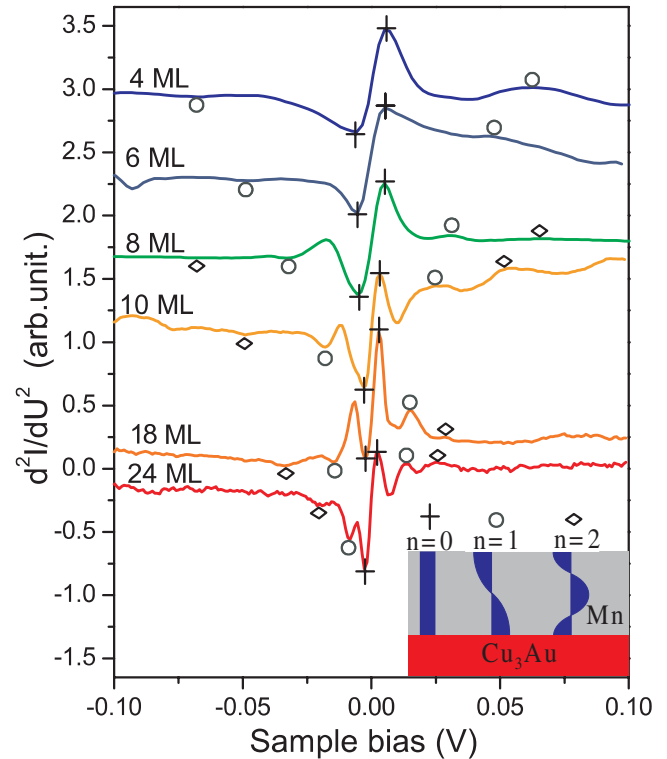
FIG. 2 (color online). d^2I/dU^2 spectra of various thicknesses Mn thin films on \text{Cu}_3\text{Au}(001) . The zero order (cross), first order (circle), and second order (parallelogram) excitation peaks are marked in the figure. These excitations correspond to standing spin waves as sketched in the inset.
