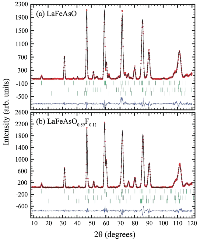
FIG. 1 (color). Neutron powder diffraction data: (a) LaFeAsO ( S 1) and (b) LaFeAsO 0.89 F 0.11 ( S 2). In both panels, the first three lines are the sample phase, aluminum sample can, and FeAs. For (a), the fourth line is La 2 O 3 while for (b), it is LaOF.
