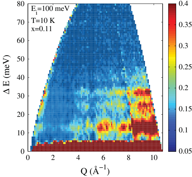
FIG. 2 (color). Inelastic neutron scattering intensity (color scale) of \text{LaFeAsO}_{0.89}\text{F}_{0.11} (S2) at 10 K as a function of Q and E . The scattering due to the empty sample holder has been removed.
