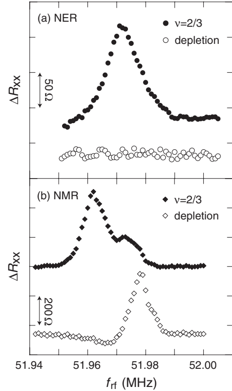
FIG. 2. (a) NER spectrum of ^{75}\text{As} for the \nu = 2/3 system (solid circles). \Delta R_{xx} caused by the rf electric field of \tau_{rf} = 1 s and P_{rf} = -15 dBm is plotted as a function of f_{rf} . \Delta R_{xx} at depletion (open circles) is also plotted. (b) Resistively-detected NMR spectra of ^{75}\text{As} for the \nu = 2/3 system (solid diamonds) and at depletion (open diamonds) obtained by the irradiation of the rf magnetic field of \tau_{rf} = 300 ms and P_{rf} = 10 dBm. Traces are vertically offset for clarity.
