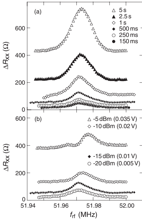
FIG. 3. NER spectra of ^{75}\text{As} for the \nu = 2/3 system for several values of (a) \tau_{\text{rf}} at P_{\text{rf}} = -15 dBm and (b) P_{\text{rf}} at \tau_{\text{rf}} = 500 msec, respectively. The amplitude of the bias modulation for each P_{\text{rf}} is shown inside the parentheses.
