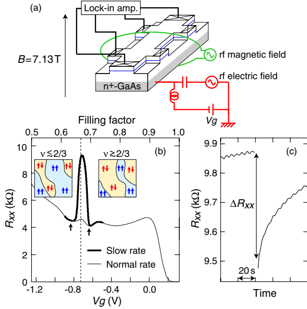
FIG. 1 (color online). (a) Schematic of the experimental setup. (b) R_{xx} at B = 7.13 T obtained by sweeping the gate bias at normal ( dV_g/dt = 5.0 \times 10^{-3} V/s) and slow ( dV_g/dt = 5.0 \times 10^{-5} V/s) sweep rates. The filling factor is shown on the top axis. The dotted line represents \nu = 2/3 . Arrows point to R_{xx} minima for the spin-polarized and -unpolarized states. Insets show illustrations of domain structures for filling factors slightly higher and lower than \nu = 2/3 , where the spin-unpolarized and -polarized states are dominant, respectively. (c) Time evolution of R_{xx} at \nu = 2/3 ( V_g = -0.74 V). The resistance drop is caused by the burst of the rf electric field at 51.971 MHz. The burst duration and the output power of the rf generator are \tau_{rf} = 1 s and P_{rf} = -15 dBm, respectively.
