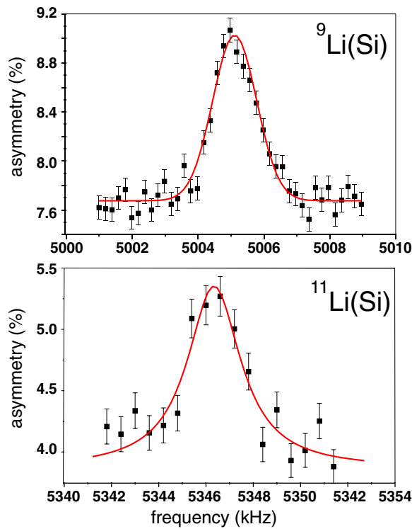
FIG. 1 (color online). NMR resonances for {}^9\text{Li} and {}^{11}\text{Li} in a Si crystal.
