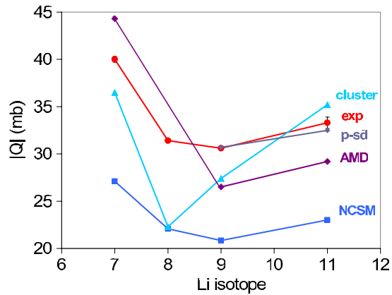
FIG. 4 (color online). Quadrupole moments of the Li isotopes compared to values from different theoretical models.
