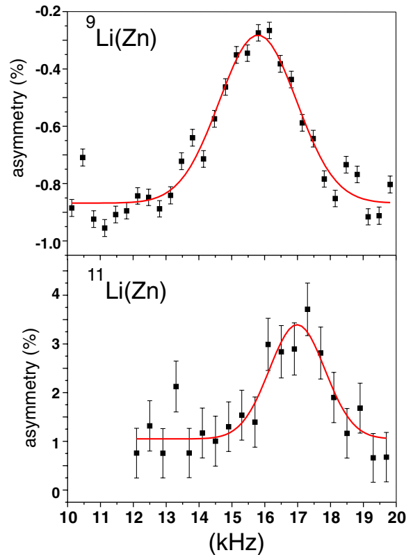
FIG. 2 (color online). Multiple-rf resonances for {}^9\text{Li} and {}^{11}\text{Li} in a Zn crystal.
