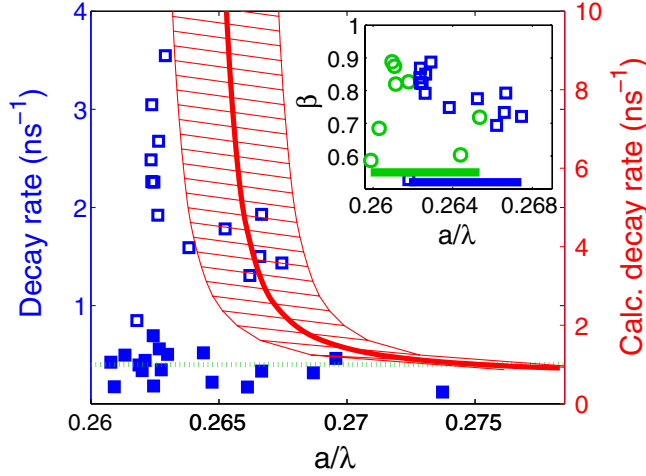
FIG. 4 (color online). Measured decay rates for QDs in a PCW sample with a = 248 nm. The pump excitation power was 1.5 kW/cm 2 . The data points marked by open (solid) squares are modeled using a double (single) exponential decay model. The red line (right axis) shows the decay rates calculated from numerical simulations with uncertainties in a of \pm 2 nm given by the hatched area. The dotted green line is the mean decay rate of uncoupled QDs used for the estimation of \beta . The inset displays the \beta -factors above 0.5 calculated from the data in Fig. 3 (green circles) and Fig. 4 (blue squares) as described in the text. The green (blue) bar shows the coupling bandwidth of the PCW sample with a = 256 nm ( a = 248 nm).
