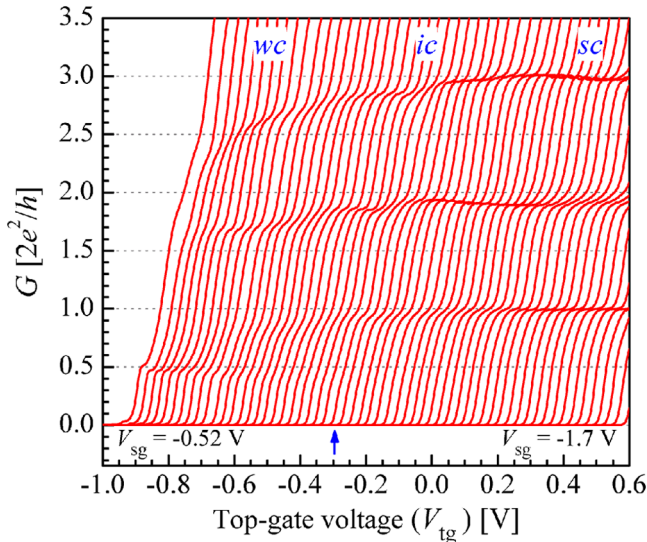
FIG. 1 (color online). Differential conductance G(V_{tg}) measured at T = 50 mK with fixed V_{sg} , ranging from -1.7 V on the right-hand side to -0.52 V on the left-hand side. A structure evolves at e^2/h on the left-hand side accompanied by the suppression of the 2e^2/h degenerate plateau. Moving from right to left sc , ic , and wc mark the strong-, intermediate-, and weak-confinement regimes described in the text. The arrow at the bottom of the figure indicates the onset of a plateau at e^2/h , corresponding to the arrow shown in Fig. 2.
