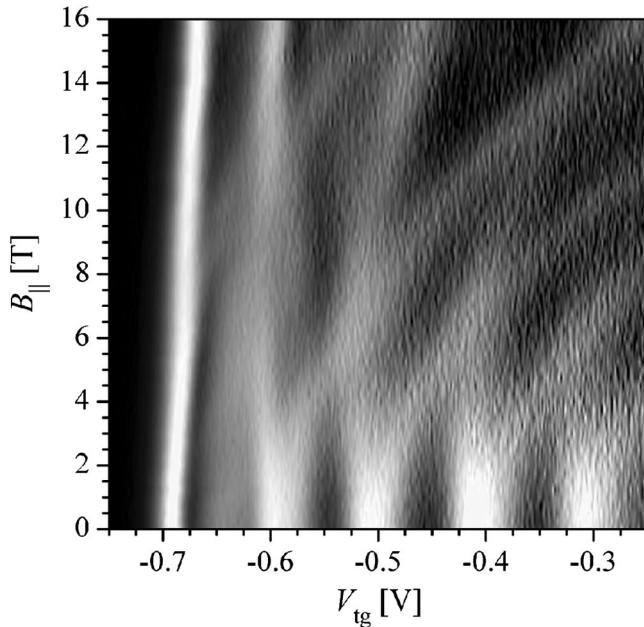
FIG. 4. Gray-scale plot of dG/dV_{\text{tg}} with B_{\parallel} . Diverging pairs of light lines for V_{\text{tg}} > -0.62 V indicate Zeeman splitting for subbands N \geq 2 . The sharp light line on the left-hand side at V_{\text{tg}} = -0.69 V corresponds to spin-incoherent electrons. It appears to be the spin-split branch of N = 1 ; however, note that at 9 T, a branch comes out to the right of this line, at which point the transport becomes spin coherent.
