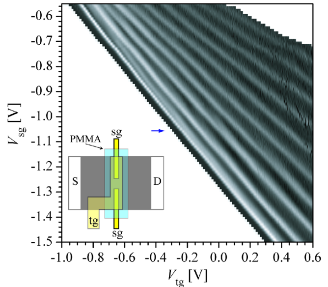
FIG. 2 (color online). Gray-scale plot of transconductance dG/dV_{tg} . Gradual suppression of the 2e^2/h plateau and strengthening of the e^2/h plateau are marked by a thin light line bridging the two adjacent light lines at the bottom. Inset : Schematic diagram of the device (not to scale) showing the split gates ( sg ) and top gate ( tg ) separated by a dielectric layer ( PMMA ).
