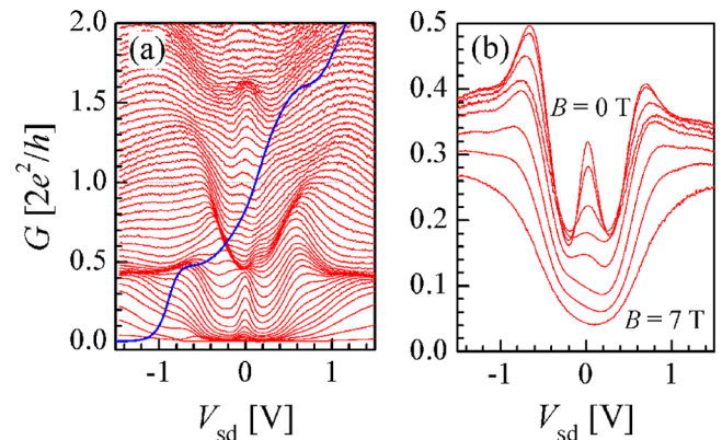
FIG. 5 (color online). (a) G(V_{\text{sd}}) showing a zero-bias anomaly peak for G < e^2/h and its suppression above e^2/h . (b) G(V_{\text{sd}}) measured at fixed B_{\parallel} . The ZBA shows no discernible splitting up to B_{\parallel} = 7 T, beyond which the peak is completely suppressed.
