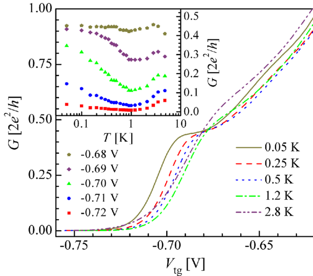
FIG. 6 (color online). Dependence of the e^2/h plateau on the lattice temperature. There is overall thermal averaging, a 0.7 structure evolves at higher T . Inset: Temperature dependence of G at various carrier densities ( V_{\text{tg}} ); the top trace is for the midpoint of the plateau.
