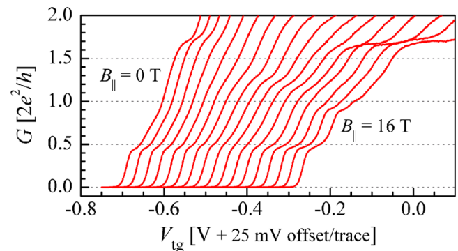
FIG. 3 (color online). Differential conductance G(V_{tg}) in the wc regime at fixed B_{||} , incremented from 0 to 16 T in steps of 1 T. The e^2/h plateau initially weakens up to 9 T, but no appreciable change in the quantized value is observed.
