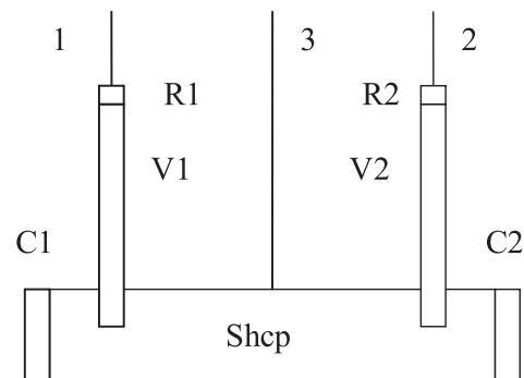
FIG. 1. Schematic of the apparatus. Vycor rods V1 , V2 enter the copper sample cell, with solid sample \text{Shcp} (4.45 cm long, 0.64 cm diam), which has capacitive pressure gauges C1 , C2 and is cooled from the bottom. Thermometers are located on the cell and at the reservoirs R1 , R2 . The pressures in lines 1 and 2 are recorded at room temperature.
