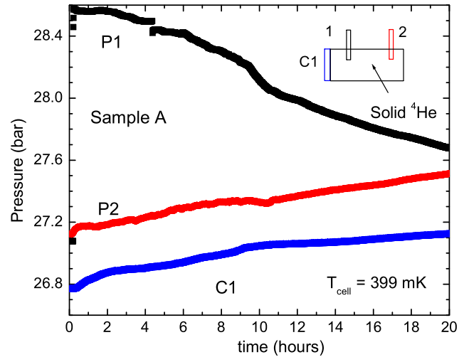
FIG. 2 (color online). Response of the apparatus to a pressure step applied to line 1 for sample A, grown at 26.8 bar. The shift in P1 just after 4 h is an artifact from the fill of a nitrogen trap. The regulator, which controls the pressure that feeds line 1, was shut off at 6 h. The pressure increase in line 2 was essentially linear in time, especially for the final 10 h.
