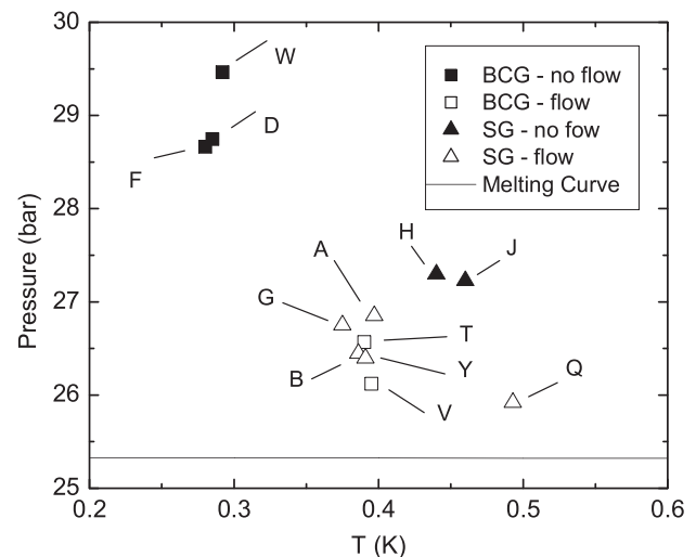
FIG. 4. Phase diagram depicting some of the locations for which we have made samples. BCG is blocked capillary growth, SG is growth from the superfluid at constant temperature. Solid symbols indicate samples for which no flow was observed. Letters denote samples; some are mentioned in the text while others and more detail are available [25].
