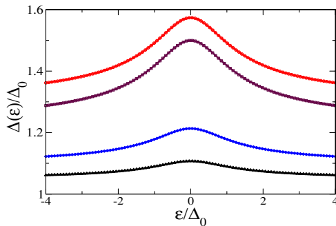
FIG. 1 (color online). Superconducting order parameter \Delta(\epsilon) in units of the bulk gap \Delta_0 for chaotic Al grains ( k_F = 17.5 \text{ nm}^{-1} , \delta = 7279/N , \Delta_0 \approx 0.24 \text{ meV} ) as a function of energy \epsilon counted from the Fermi level. Different curves correspond to grain sizes (top to bottom) L = 6 \text{ nm} , k_F L = 105 , \delta/\Delta_0 = 0.77 (Dirichlet and Neumann boundary conditions), L = 8 \text{ nm} , k_F L = 140 , \delta/\Delta_0 = 0.32 (Dirichlet), and L = 10 \text{ nm} , k_F L = 175 , \delta/\Delta_0 = 0.08 (Dirichlet). The leading contribution comes from the energy dependent matrix elements I(\epsilon, \epsilon') obtained from Eqs. (5) and (6). Note that the order parameter is always larger than its bulk value \Delta_0 and has a single maximum at the Fermi level.
