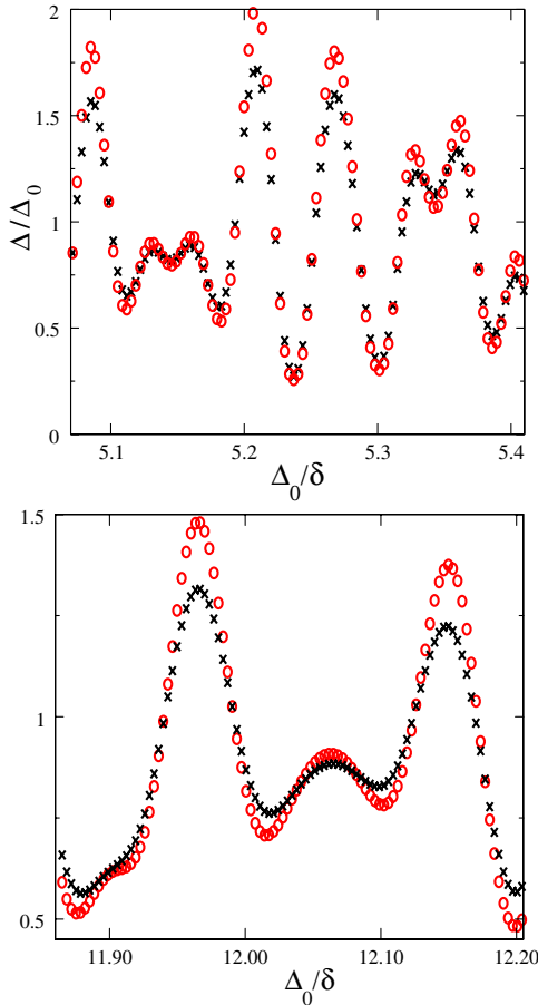
FIG. 2 (color online). Superconducting order parameter \Delta in units of the bulk gap \Delta_0 for a cubic Al grain as a function of the ratio \Delta_0/\delta , where \delta is the mean level spacing. Black crosses correspond to the exact numerical solution of the gap Eq. (2), while the red circles represent the semiclassical analytical expression.
