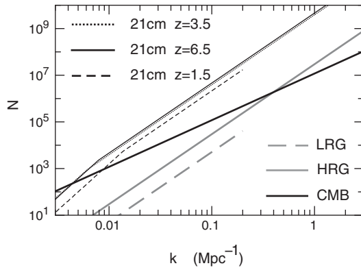
FIG. 2. The number of modes N within a wave number bin of width \Delta k = k/10 centered on k that are available in different cosmological surveys. The thick dashed gray line corresponds to the spectroscopic LRG sample of SDSS [16], while the thick solid line (marked HRG for “high redshift galaxies”) corresponds to a future spectroscopic survey at 2.5 < z < 3.5 covering 1000 square degrees with a comoving galaxy density equal to the LRG sample. The thick dark line corresponds to a CMB data set with f_{\text{sky}} = 0.65 . The thin lines show the number of modes accessible in a 21 cm survey (including the limit on large-scale modes due to foreground removal [12]) covering f_{\text{sky}} = 0.65 within a redshift range spanning a factor of 3 in (1+z) , and centered on z = 1.5, 3.5, and 6.5 . For z \leq 1.5 , we have truncated the curves at k = 0.2 \text{ Mpc}^{-1} to illustrate the smaller range of k accessible within the linear regime at lower redshifts [33].
