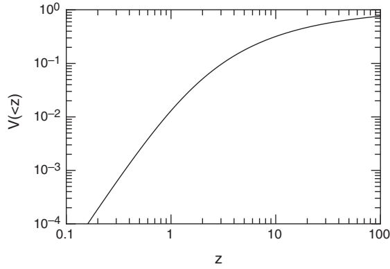
FIG. 1. The fraction of the total comoving volume of the observable Universe that is available up to a redshift z .
