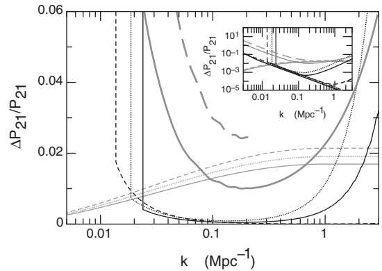
FIG. 3. The fractional change in the amplitude of the power spectrum owing to the presence of a massive neutrino (horizontal gray lines, asymptoting towards a constant at high k values). The case shown, f_\nu = 0.004 , corresponds to m_\nu = 0.05 \text{ eV} . For comparison, the limits imposed by cosmic variance on measurements of the power spectrum from the SDSS-LRG and a future 1000 square degree galaxy survey at 2.5 < z < 3.5 are marked by the thick dashed and solid gray lines, respectively. The U -shaped error curves correspond to an all-sky 21 cm survey [ f_{\text{sky}} = 0.65 over a redshift range spanning a factor of 3 in (1+z) ] with MWA5000 and a 10^3 \text{ h} integration per field (line styles for z = 1.5, 3.5, 6.5 as in Fig. 2). The noise is plotted in bins of size \Delta k/k = 0.1 . The inset shows these results on logarithmic axes that span a larger dynamic range of achievable precision. The straight thin lines in the inset show the cosmic-variance uncertainty in the power-spectrum measurement owing only to the number of available modes. For z \leq 1.5 , we have truncated the curves at k = 0.2 \text{ Mpc}^{-1} to illustrate the smaller range of k accessible within the linear regime at lower redshifts [33].
