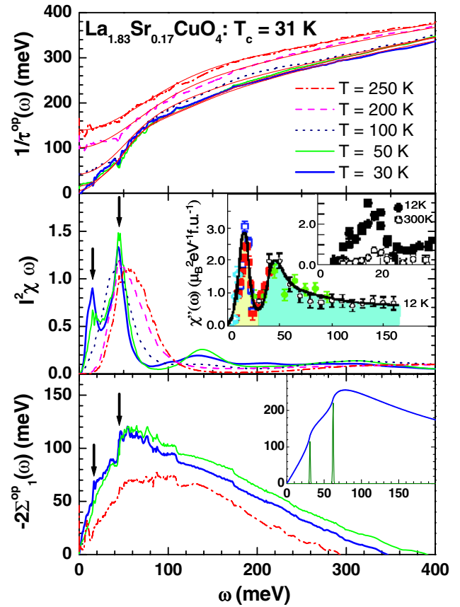
FIG. 1 (color online). Top panel: The optical scattering rate 1/\tau^{\text{op}}(\omega) in meV as a function of \omega (in meV) for five temperatures. The heavy lines are the experimental data (TO phonons have been subtracted to isolate the electronic contribution). The light solid lines are the fits to the data. Middle panel: The electron-boson spectral density I^2\chi(\omega) obtained from our Eliashberg inversion from the data in the top panel. The inset shows the data of Vignolle et al. for a closely related sample of \text{La}_{2-x}\text{Sr}_x\text{CuO}_4 with x = 0.16 and T_c = 38.5 K. In the inset of the inset the data with solid points are at 12 K and a comparison with 300 K data below 40 meV is also given (open points). Bottom panel: The real part of the optical self-energy \Sigma_1^{\text{op}}(T, \omega) for LSCO. The arrows show the positions of the sharp peaks found in the spectral density at low temperature, \omega = 15 and \omega = 44 meV. Note the sharp rise in the self-energy at these frequencies. In the inset we show a simulated self-energy using a mode with two Einstein modes.
