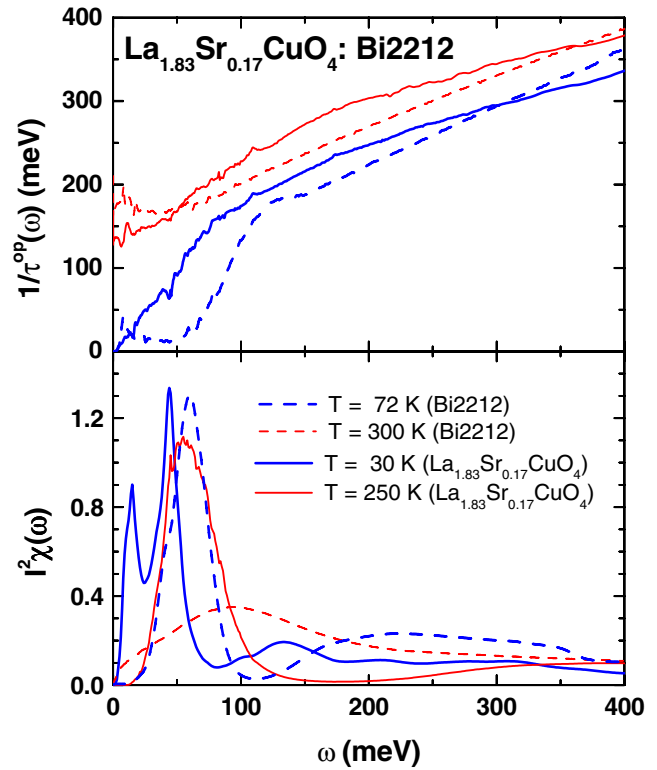
FIG. 2 (color online). Top panel: Scattering rates for Bi-2212 (dashed lines) and LSCO (solid lines). The two materials show striking differences at low energies. Scattering sets in at very low energies in the LSCO material whereas Bi-2212 has a negligible scattering below 50 meV. Bottom panel: The bosonic spectral function I^2\chi(\omega) of the same materials shown in the top panel. At low temperature LSCO has two peaks while Bi-2212 shows a single peak at much higher energy. As the temperature is raised the Bi-2212 peak is weakened dramatically and moves to high frequency [25] whereas in LSCO the lower peak vanishes while the upper peak remains up to 250 K. This difference at high temperature can already be seen in the top panel: the LSCO sample shows an onset of scattering in the 50 meV region while the Bi-2212 curve is quite featureless at 300 K.
