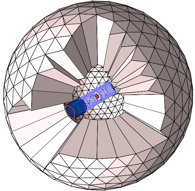
FIG. 1 (color online). Diagram showing the Crystal Ball detector, the cylindrical {}^{12}\text{C} target at the center of the detector [dark gray (red)] and the PID detector components [light/dark gray (blue)] surrounding the target. The MWPC is omitted for clarity.
