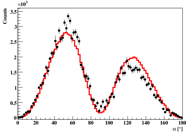
FIG. 4 (color online). Comparison of the distribution of \alpha , the polar angle of the nuclear decay photon with respect to the recoil direction, for incident E_\gamma = 235 \pm 10 MeV (black points) with the distribution suggested in Ref. [2], passed through the G3 simulation of the experimental acceptance (solid red line).
