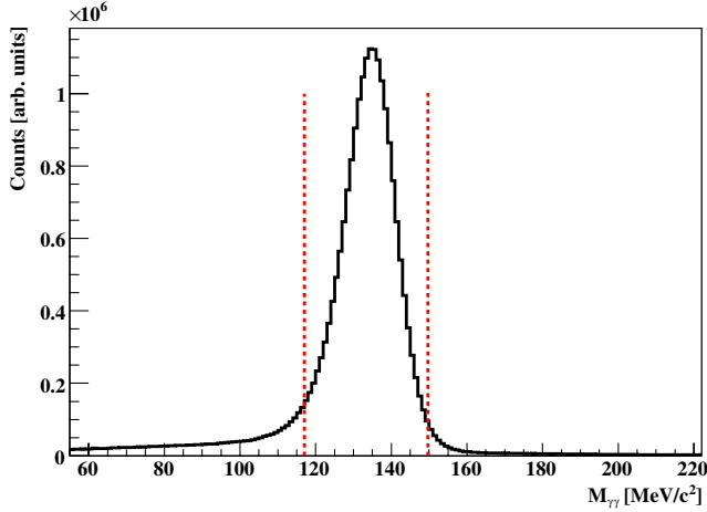
FIG. 2 (color online). The spectrum of invariant mass reconstructed from the 2\gamma events in the CB for E_\gamma \leq 400 MeV. Events in the mass range 117–149 MeV were selected for the analysis.
