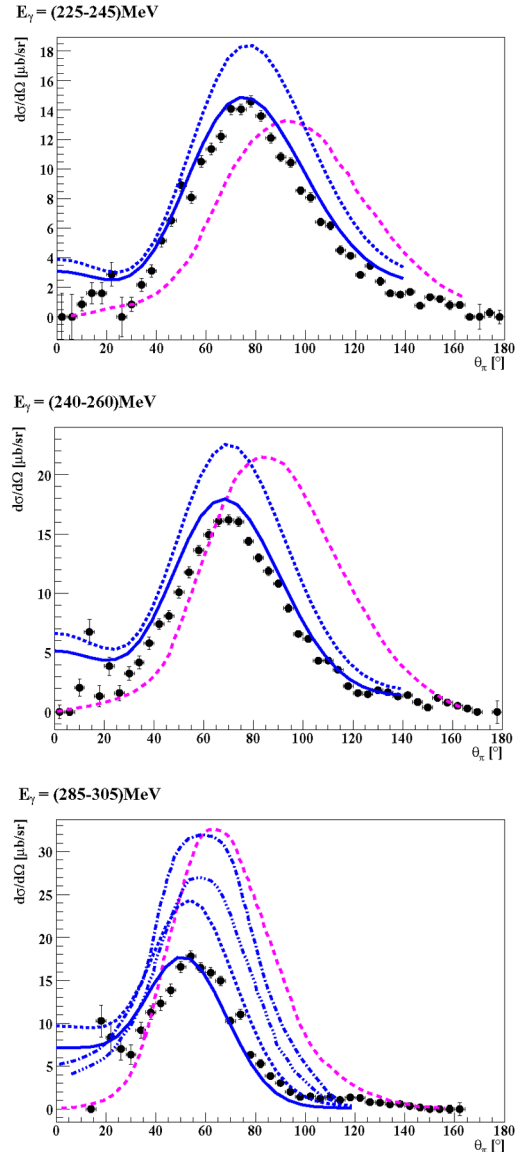
FIG. 5 (color online). The ^{12}\text{C}(\gamma, \pi^0)^{12}\text{C}_{4.4 \text{ MeV}} cross section presented as a function of \theta_\pi for E_\gamma bins indicated in the figure. The predictions by Takaki et al. [1,23] are shown by dark gray (blue) lines: distorted-wave impulse approximation (dot-dashed line); many body effects added (dot-dot-dashed line); multistep mechanisms also added (dashed line); \Delta - N interaction also added (solid line). Light gray (pink) long dashed line shows predictions of Ref. [2].
