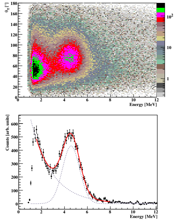
FIG. 3 (color online). Top: \theta_\pi versus the energy of the low-energy clusters detected in the CB. Bottom: Projection of the energy distribution for \theta_\pi bin of 78 \pm 2^\circ . The gray dotted lines show the result of an exponential plus Gaussian fit to the data. Both plots for E_\gamma = 235 \pm 10 MeV and for E_\pi^{\text{diff}} below 20 MeV.
