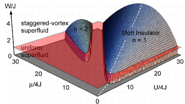
FIG. 1 (color online). Phase diagram with respect to the chemical potential \mu , the interaction parameter U , the hopping amplitude J , and the scaled magnetic flux W . Within the three-dimensional lobes a gapped Mott-insulator phase prevails. Outside these lobes the system is superfluid. For small magnetic fields ( W/J < 1 ) the superfluid is spatially uniform, while for large magnetic fields ( W/J > 1 ), a quantized staggered rotational flux arises. The white dashed line indicates the (\mu/U = 2 - \sqrt{2}) plane analyzed in detail in Fig. 2.
