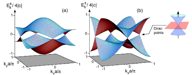
FIG. 3 (color online). Single-particle spectrum for (a) \theta < \pi/4 , with the minimum at the origin, and (b) \theta > \pi/4 , with minima at the Brillouin zone edges (\pm \pi/a, \pm \pi/a) .
