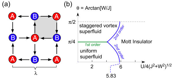
FIG. 2 (color online). (a) The bipartite lattice comprises sites labeled by “A” and “B.” The gray rectangle identifies a single plaquette. The solid arrows indicate the tunnelling currents driven by V_R(\mathbf{r}, t) . (b) Phase diagram within the (\mu/U = 2 - \sqrt{2}) plane spanned by the dashed white line and the W axis in Fig. 1.
