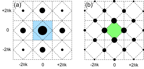
FIG. 4 (color online). Schematic of the momentum spectra for the uniform superfluid (a) and the staggered-vortex superfluid (b). The colored areas in the centers illustrate the first Brillouin zones with (b) and without (a) the staggered magnetic field.
