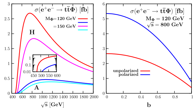
FIG. 2 (color online). The production cross sections \sigma(e^+e^- \rightarrow t\bar{t}\Phi) for a scalar and a pseudoscalar Higgs boson as a function of \sqrt{s} for two masses M_\Phi = 120 and 150 GeV (left) and for unpolarized and polarized e^\pm beams as a function of the parameter b at \sqrt{s} = 800 GeV with M_\Phi = 120 GeV (right). The inset in the left panel shows the region near the threshold in more detail.
