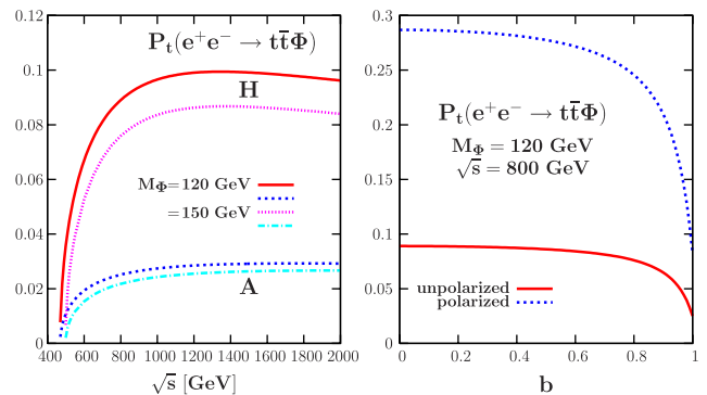
FIG. 3 (color online). The top quark polarization in the process e^+e^- \rightarrow t\bar{t}\Phi for a scalar and a pseudoscalar Higgs boson as a function of \sqrt{s} for two masses M_\Phi = 120 and 150 GeV (left) and with unpolarized and polarized e^\pm beams as a function of the parameter b at \sqrt{s} = 800 GeV for M_\Phi = 120 GeV (right).
