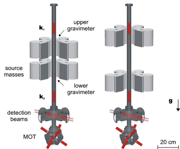
FIG. 1 (color online). Schematic of the experiment showing the gravity gradiometer setup with the Raman beams propagating along the vertical direction. During the G measurement, the position of the source masses is alternated between configuration C_1 (left) and C_2 (right).
