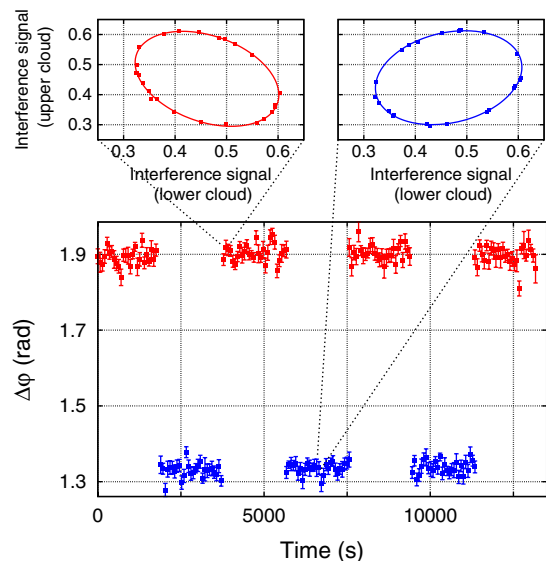
FIG. 3 (color online). Typical data set showing the modulation of the differential phase shift measured by the atomic gravity gradiometer when the distribution of the source masses is alternated between configuration C_1 (upper points) and C_2 (lower points). Each phase measurement is obtained by fitting a 24-point scan of the atom interference fringes to an ellipse.
