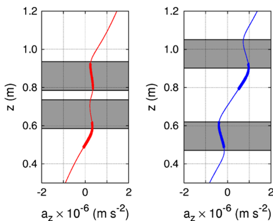
FIG. 2 (color online). Acceleration along the symmetry axis of the system in configuration C_1 (left) and C_2 (right). The simulation includes the effect of the source masses and the Earth's gravity gradient. The spatial extension of the atomic trajectories for the upper and lower interferometers is indicated by the thick lines. The shaded regions show the positions of the source masses.
