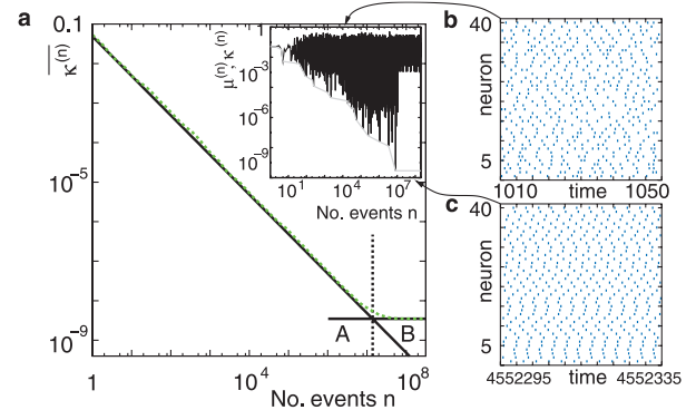
FIG. 2 (color). Convergence towards a periodic orbit in a random network ( N = 40 , \gamma_i^{-1} \equiv 1.0 , I_i \equiv 3.0 , \phi_{\Theta,i} \equiv 1.0 , \tau_{i,j} \equiv 0.1 , p = 0.2 , \sum_j \varepsilon_{i,j} \equiv -3.3 ). (a) The average minimal margin \overline{\kappa^{(n)}} [as in Fig. 1(c)] decays as a power law (region A) and saturates after about 10^7 events (region B) when the periodic orbit is reached. Inset: Margin \mu^{(n)} (black) and minimal margin \kappa^{(n)} (gray) for a trajectory started from one specific initial condition. The margin \mu^{(n)} fluctuates strongly on the transient; after the sequence becomes periodic the minimal margin \kappa^{(n)} does not decrease further for future events n . (b), (c) Snapshots of (b) irregular spike sequences after n \approx 2 \times 10^4 events on the transient and (c) after n \approx 10^8 events on the periodic orbit.
