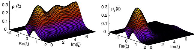
FIG. 1 (color online). Quenched density \rho_1(\xi) of Eq. (10) (left), and quenched p_1(\xi) from Eq. (6) (including the first three terms) for circular J (right), both for \nu = 0 and \alpha = 0.174 .
