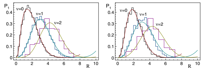
FIG. 3 (color online). Integrated distribution P_1(R) = \int_0^\pi d\theta R p_1(R, \theta) of the first eigenvalue for \nu = 0, 1, 2 as a function of the radius R for \mu = 0.1 (left) and \mu = 0.2 (right). The solid lines are the RMT results from Eq. (6), the histograms are the quenched lattice data of Ref. [24]. The bending-up of the RMT curves for large R is an artifact of using only the first three terms in the expansion (6), see text.
