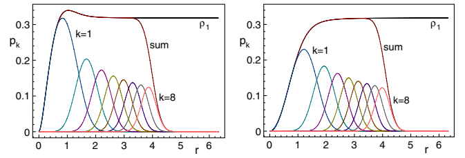
FIG. 2 (color online). Quenched spectral density Eq. (11) and distributions of the first eight eigenvalues Eq. (13), as well as their sum, all in the large- \alpha limit, for \nu = 0 (left) and \nu = 1 (right).
