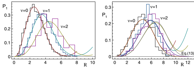
FIG. 4 (color online). Same as Fig. 3, but for \mu = 0.3 (left) and \mu = 1.0 (right). For \mu = 1.0 , we also show the exact RMT result in the large- \alpha limit from Eq. (13).
