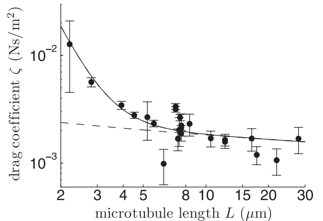
FIG. 4. Drag coefficients \zeta versus contour length L . For short microtubules, the experimental data lie significantly above the hydrodynamic estimate \zeta_0 of Eq. (2) (dashed line). The solid line shows a fit of Eq. (7) taking into account internal friction.
