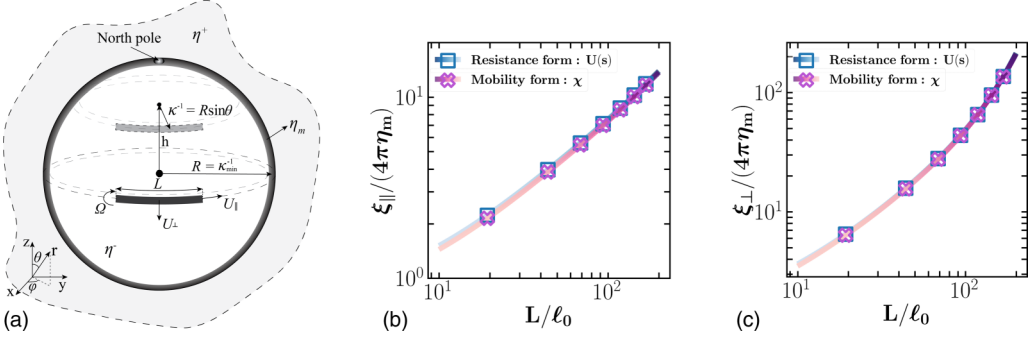
FIG. 1. (a) An illustration of the filament motion on a spherical membrane of viscosity \eta_m and surrounded on the interior and exterior sides by 3D fluid domains of shear viscosities \eta^- and \eta^+ . The filament dynamics is described by three modes of motion: translation along and perpendicular to its axis ( U_{\parallel} and U_{\perp} ), and rotation ( \Omega ). The filament's curvature is at its minimum when it is aligned along the equator ( \kappa_{\min} = R^{-1} ). The results of this configuration are presented in Sec. IV A. To model filaments of curvature \kappa > \kappa_{\min} , they are placed at distance h = \pm\sqrt{R^2 - \kappa^{-2}} away from the equator. This configuration is studied in Sec. IV B. (b, c) The dimensionless resistance of a filament translating in parallel (b) and perpendicular (c) directions as a function of L/\ell_0 , where \ell_0/R = 0.01 . The blue line (square dots) shows the result of the numerical solutions to the resistance formulation given by \mathbf{U}(s) , Eq. (4), while the red line (cross dots) shows the numerical integration of the mobility formulation given by \chi , Eq. (5), assuming a constant force density along the filament. The results are in excellent agreement with each other.
