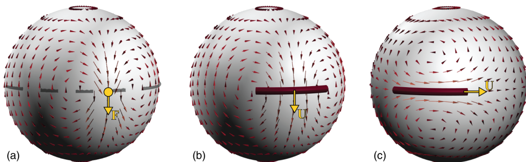
FIG. 3. (a) The flow field induced by a point force in the perpendicular direction at (\theta = \pi/2, \phi = 0) for the choice of \ell_0/R = 1 . (b) The flow field induced by a filament moving with a constant velocity in the perpendicular direction for the choice of \ell_0/R = 1 and L/R = 1 . (c) The flow field induced by a filament moving with a constant velocity in the parallel direction for the choice of \ell_0/R = 1 and L/R = 1 .
