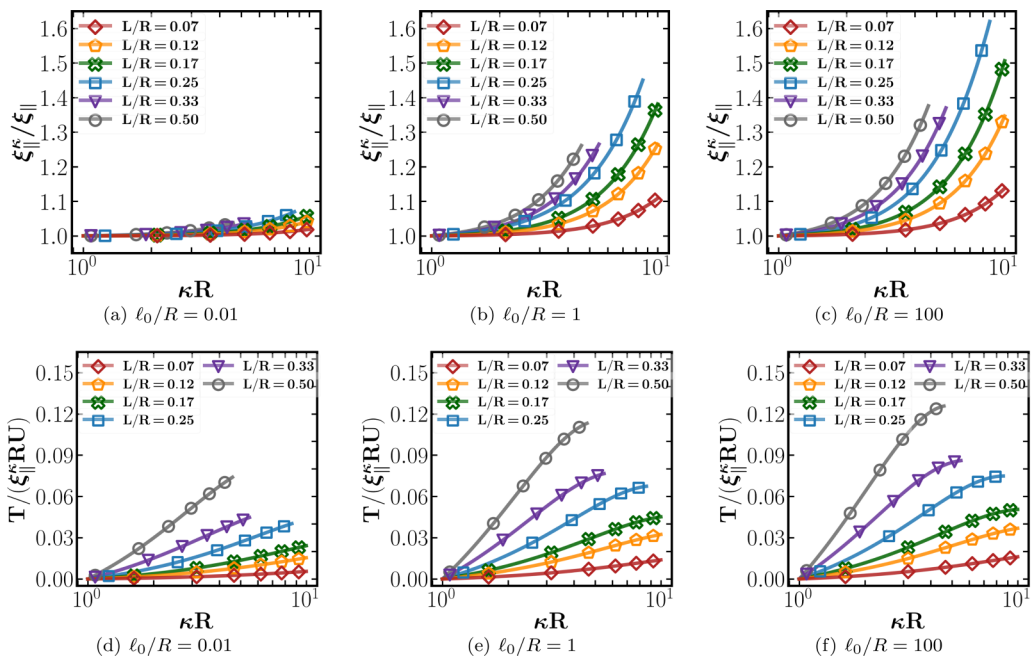
FIG. 6. Top row (a–c) The resistance along the parallel direction vs the filament’s dimensionless curvature ( \kappa R ) for 0.07 \leq L/R \leq 0.50 at (a) l_0/R = 0.01 , (b) l_0/R = 1 , and (c) l_0/R = 100 . When l_0/R \ll 1 the parallel resistance remains nearly constant with curvature and equal to the results at the equator. When l_0/R \geq 1 , the resistance monotonically increases with curvature, and the rate of this increase is amplified with increasing L/R . Bottom row (d–f): the net torque induced on the filament by its motion in the parallel direction as a function of the filament’s dimensionless curvature for the range 0.07 \leq L/R \leq 0.50 at (d) l_0/R = 0.01 , (e) l_0/R = 1 , and (f) l_0/R = 100 . The torque magnitude is nondimensionalized by the external force moment on the membrane: \xi_{\parallel}^{\kappa} R U . Regardless of the choice of l_0/R , the torque monotonically increases with \kappa R ; this effect is amplified with increasing L/R . The results appear to be a weak function of l_0/R , and the torque remains < 15\% of the external force moment.
