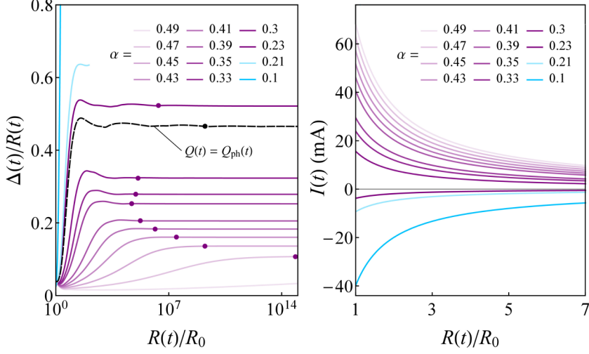
FIG. 2. Left panel: Behavior of the shape factor \Delta(t)/R(t) with respect to variations in the ratio R(t)/R_0 , for flows performed utilizing the controlling protocol with n_{\max} = 7 and various injection rates Q(t) = \alpha Q_{\text{crit}}(t) . Right panel: Plot of the electric current Eq. (5) as a function of R(t)/R_0 for the injection rates utilized in the left panel.
