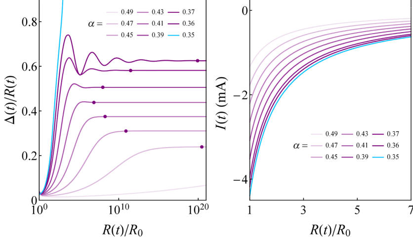
FIG. 4. Left panel: Behavior of the shape factor \Delta(t)/R(t) with respect to variations in the ratio R(t)/R_0 , for flows performed utilizing the controlling protocol with n_{\max} = 3 and various injection rates Q(t) = \alpha Q_{\text{crit}}(t) . Right panel: Plot of the electric current Eq. (5) as a function of R(t)/R_0 for the injection rates utilized in the left panel.
