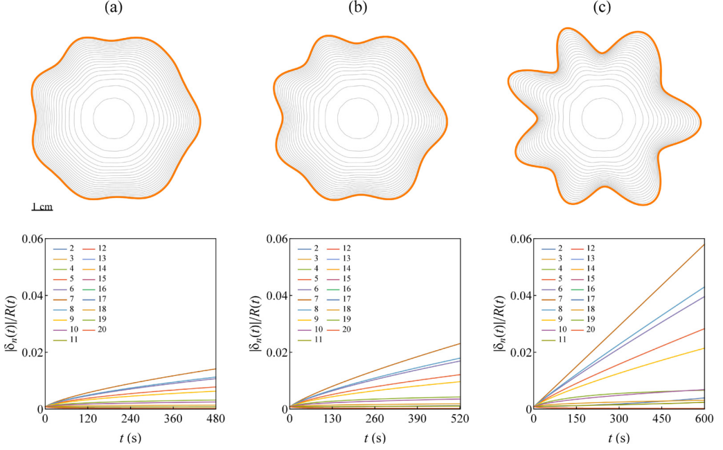
FIG. 7. Weakly nonlinear time evolution of the expanding interfacial patterns generated by utilizing the controlling protocol for n_{\max} = 7 , and three injection rates Q(t) = \alpha Q_{\text{crit}}(t) : (a) \alpha = 0.25 , (b) \alpha = 0.23 , and (c) \alpha = 0.2 . Here we include modes 2 \leq n \leq 20 and a random initial phase. The corresponding time evolution of the rescaled perturbation mode amplitudes |\delta_n(t)|/R(t) are shown in the bottom panels. The final times used are (a) t_f = 480 s, and (b) t_f = 600 s, and the remaining physical parameters are listed in Table I.
