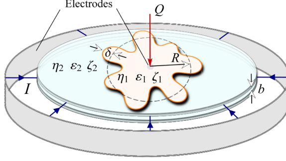
FIG. 1. Representative sketch of the electrohydrodynamic Hele-Shaw flow.
