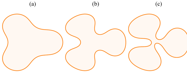
FIG. 5. Gallery of representative fully nonlinear threefold patterns corresponding to the cases (a) \alpha = 0.45 , (b) \alpha = 0.37 , and (c) \alpha = 0.35 , shown in Fig. 4. The interfaces (a) and (b) are plotted at the onset of the self-similar regime, i.e., for (a) R/R_0 = 8.2 \times 10^{10} and (b) R/R_0 = 3.2 \times 10^{11} . The pattern depicted in (c) does not reach the self-similar regime, and is plotted for R/R_0 = 1.06 \times 10^3 .
