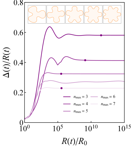
FIG. 6. Behavior of the shape factor \Delta(t)/R(t) with respect to variations in the ratio R(t)/R_0 , for flows performed utilizing the controlling protocol with n_{\max} = 3, 4, 5, 6 , and 7 . Here Q(t) = 0.37 \times Q_{\text{crit}}(t) , where Q_{\text{crit}}(t) is evaluated for each mode n_{\max} utilizing Eq. (6). The resulting self-similar shapes are depicted as insets.
