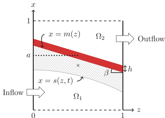
FIG. 2. Dimensionless filtration-module domain (x, z) \in \{[0, 1] \times [0, 1]\} . The membrane and cake layers are schematized in red and gray, respectively, with the evolved cake front denoted by x = s(z, t > 0) . The membrane center is at (x, z) = (a, 1/2) and is specified by the parameter a . The membrane angle is given by \beta .
