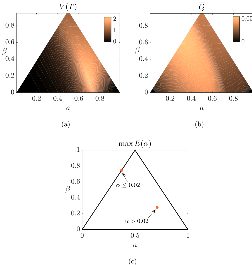
FIG. 6. The total throughput V(T) (2.38) in (a), \bar{Q} = V(T)/T in (b), and the configuration that maximizes E(\alpha) (4.2) in (c) calculated from numerical solutions to (2.36) with \beta \in [0, 1] , a \in [\beta/2, 1 - \beta/2] , \kappa_m = 1 , \phi_1^f = 0.8 , and Q_c = 10^{-2} .
