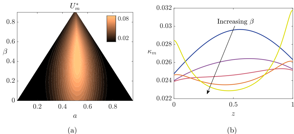
FIG. 7. The upper bound of the constant velocity U_m^* calculated in (5.5) using analytical pressure profiles (5.4) and \beta \in [0, 1] and a \in [\beta/2, 1 - \beta/2] given in (a). The nonuniform membrane permeance profiles \kappa_m(z) (5.2) calculated using (5.4) with \beta = 0, 0.2, 0.4, 0.6, 0.8 at t = 0 in (b) for a = 0.5 and U_m = 0.02 . Both figures use \phi_1^f = 0.8 .
