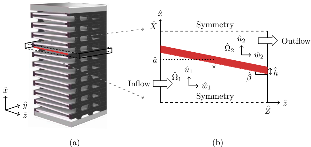
FIG. 1. Schematic of the concertinaed filtration device. (a) The full three-dimensional device; reproduced from Ref. [4] with permission. (b) The two-dimensional domain of a single filtration module; the center of the membrane is (\hat{x}, \hat{z}) = (\hat{a}, \hat{Z}/2) and the center of the domain (\hat{x}, \hat{z}) = (\hat{X}/2, \hat{Z}/2) is indicated by a cross.
