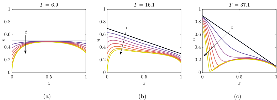
FIG. 4. Evolution of the cake profile s(z, t) over time found by solving (2.36) for \beta = 0, 0.4, 0.8 in panels (a), (b), and (c) respectively, with a = 0.5 , \phi_1^f = 0.8 , \kappa_m = k_c = 1 , Q_c = 10^{-2} . The arrows indicated the direction of growth in time, and T is the end time at which the flux Q (2.37) drops below Q_c . Results are shown for eight time steps equally spaced between [0, T] for each angle tested.
