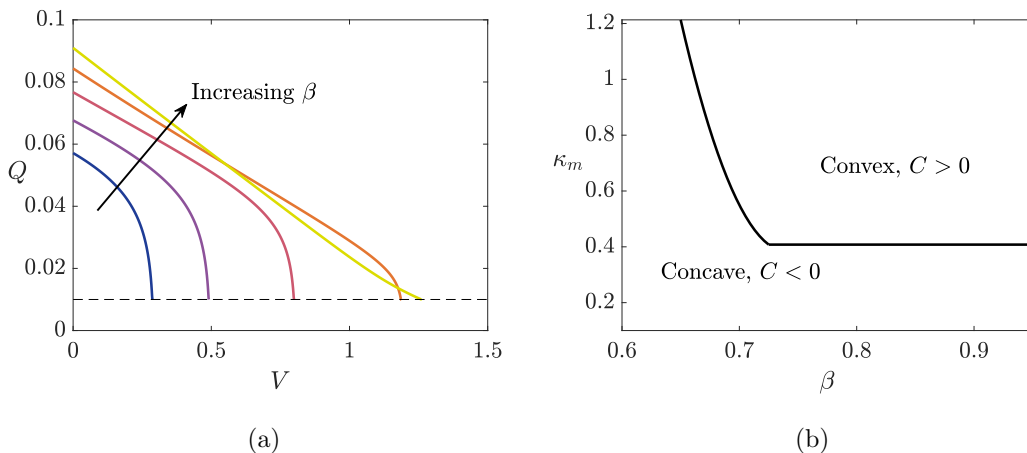
FIG. 5. Flux–throughput relationship resulting from solving the system of Eqs. (2.36) and calculating the flux Q [Eq. (2.37)] and throughput V [Eq. (2.38)] for a = 0.5 , \phi_1^f = 0.8 , \kappa_m = 1 , Q_c = 10^{-2} , and \beta = 0, 0.2, 0.4, 0.6, 0.8 in (a). Convexity C (4.1) of the flux–throughput curves indicated through \text{sgn}(C) in the (\kappa_m, \beta) domain in (b).
