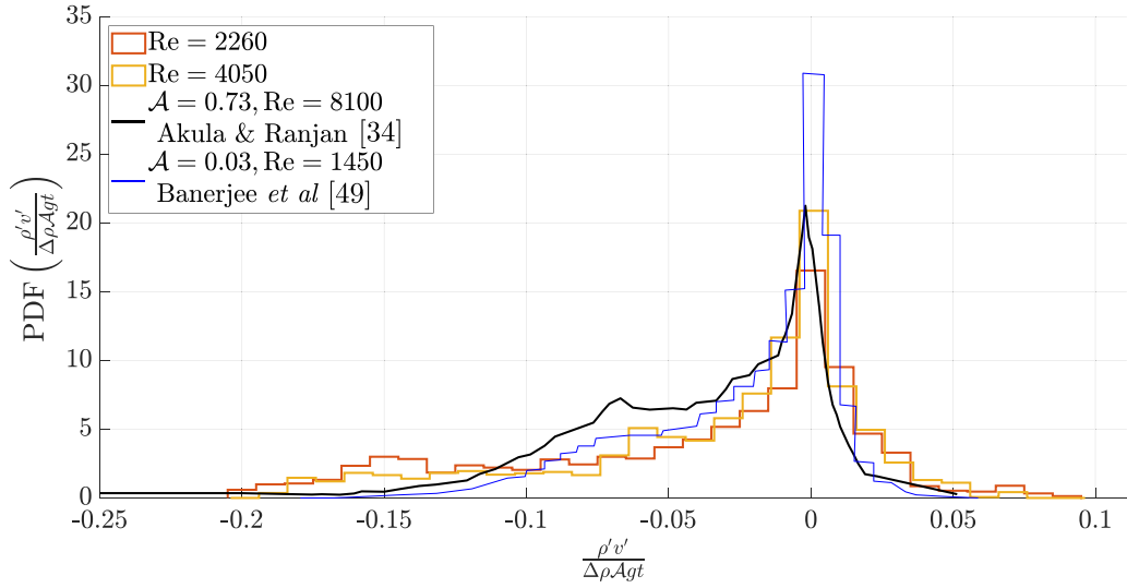
FIG. 12. The probability density function of the density-velocity correlation, \rho'v' , after normalization for the \text{Re} = 2260 and 4050 cases, evaluated at Y = 0 . To compare, the density-velocity correlation using the same normalization presented by [34,49] is shown.
