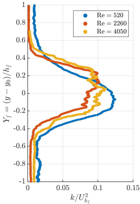
FIG. 13. Profiles of the turbulent kinetic energy, k , normalized by the self-similar velocity scale, U_{h_f} .
