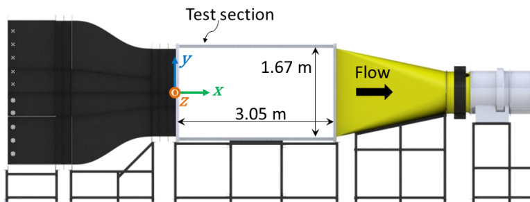
FIG. 1. 3D render of the gas tunnel facility.
