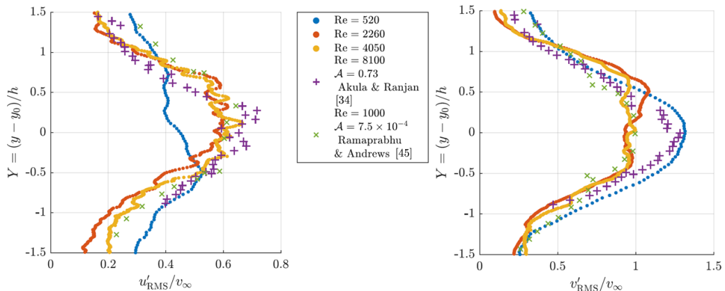
FIG. 9. Profiles of the rms horizontal and vertical velocity fluctuations, normalized by the Goncharov bubble velocity. For comparison, the normalized profiles from [34,45] are also presented.
