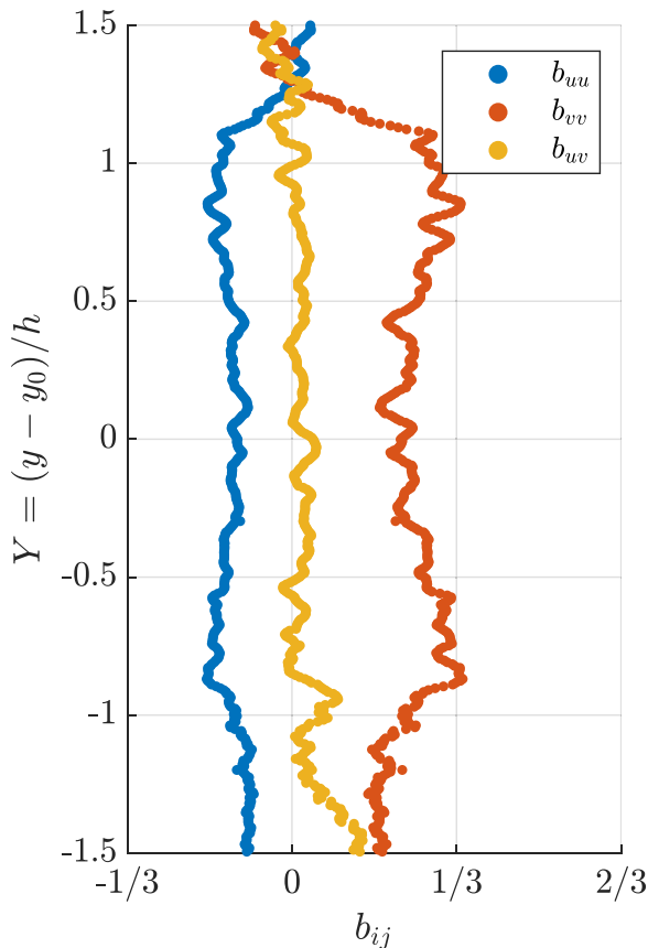
FIG. 10. Profiles of the components of the anisotropy tensor, b_{ij} , for the \text{Re} = 4050 experimental case.
