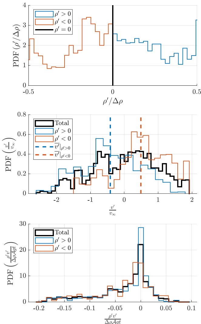
FIG. 14. Probability density functions of the normalized density, velocity, and density-velocity correlation for the sampling conditions \rho' < 0 and \rho' > 0 .
