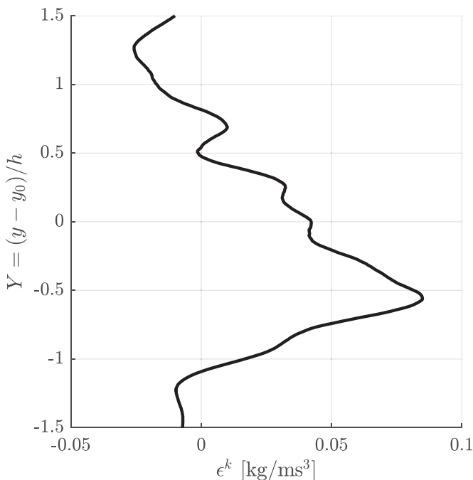
FIG. 22. Profile of the dissipation, \epsilon^k .
