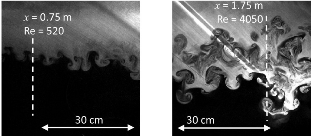
FIG. 5. Mie-scattered instantaneous images of the RTI mixing region. The vertical dashed white line indicates the position of the streamwise distance x and corresponding Re . The horizontal white line indicates a length scale of 30 cm.
