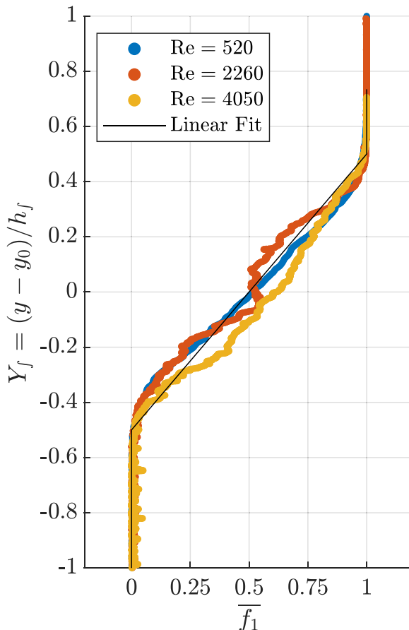
FIG. 6. Normalized profiles of the mean volume fraction of the heavy gas \bar{f}_1 for the three Reynolds numbers tested, but with the spatial coordinate normalized by h_f instead of h . Superimposed is the linear volume fraction profile assumed by [24].
