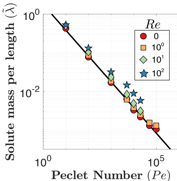
FIG. 9. Dimensionless total solute mass in the wake per unit length ( \tilde{\lambda} ), as a function of Pe , at different values of Re . Computations (points) reveal \tilde{\lambda} to be independent of Re , scaling as Pe^{-2/3} (line), irrespective of Re .
