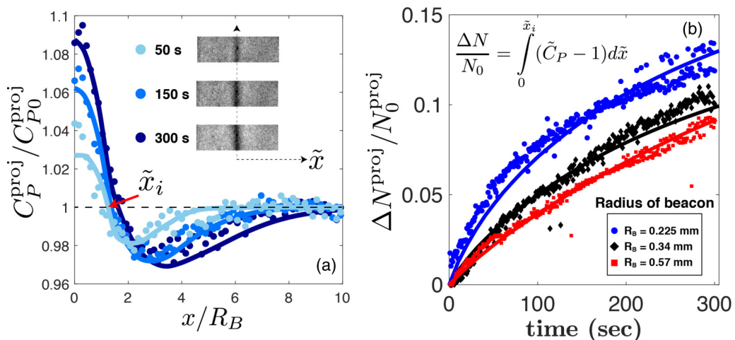
FIG. 5. Soluto-inertial attraction of suspended particles by the solute wake of a falling ionogel beacon leads to colloidal accumulation within the wake. (a) Projected concentration C_P^{\text{proj}}(x, z_0) at height z_0 in the sample cell, normalized by the background concentration C_{P0}^{\text{proj}}(x \rightarrow \infty) as a function of time. Particles migrate from the bulk suspension ( \tilde{x} > \tilde{x}_i ) to accumulate near the center of the solute wake ( \tilde{x} < \tilde{x}_i ), with intensity that increases over time. Lengths x are normalized by the beacon radius R_B , here 225 \mu\text{m} . Circle represent measured data points, and lines reflect predictions described in Sec. III. (b) The number \Delta N(t) of particles collected by the solute wake increases with time, with a collection rate that decreases with beacon radius R_B . Theoretical predictions [Eqs. (23) and (9)] capture measured data.
