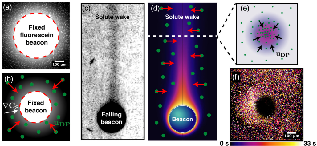
FIG. 1. Freely falling SI beacons induce diffusiophoretic colloidal migration. (a) A cylindrical beacon post fixed within a microfluidic chamber establishes a radial concentration profile of fluorescein. (b) The solute flux driven by a fixed cylindrical beacon drives suspended colloids to migrate diffusiophoretically in the radial direction. (c) Experimental visualization and (d) computed profile of solute emitted by a sedimenting beacon, which forms a convection-diffusion boundary layer along the beacon and a solute wake behind. The experiment (c) comprises a water drop unloading Oil Red O dye as it sediments through an oil bath. (e) As the solute in the wake diffuses radially outward, its concentration gradients drive suspended particles to migrate toward (or away) from the wake, creating regions in the suspension that are enriched or depleted in particles. (f) SI attraction of fluorescent colloids by a solute wake trailing a sedimenting beacon, illuminated from the side by a laser sheet and visualized from below. Color-coded streak lines show diffusiophoretic migration directed toward the center of the dark circle, which arises because the sedimenting beacon physically blocks the camera's view.
