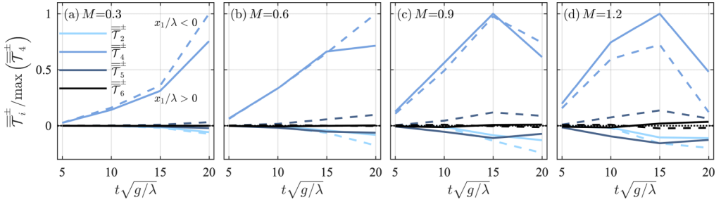
FIG. 13. Temporal dependence of half-domain averages of the dilatation, \overline{\overline{T_2}} , perturbation baroclinic torque, \overline{\overline{T_4}} , the baroclinic torque associated with background pressure, \overline{\overline{T_5}} , and the baroclinic torque associated with the background density, \overline{\overline{T_6}} , for nondimensional times t^* = t\sqrt{g/\lambda} = 5, 10, 15, and 20 and for stratification strengths M = 0.3, 0.6, 0.9, and 1.2 [(a)–(d)]. The half-domain averages used here are defined in Eqs. (38) and (39), with \overline{\overline{T_i^+}} indicating an average over x_1/\lambda > 0 (solid lines) and \overline{\overline{T_i^-}} indicating an average over x_1/\lambda < 0 (dashed lines). All results are normalized by the maximum values of the perturbation baroclinic torque over both halves of the domain for each M .
